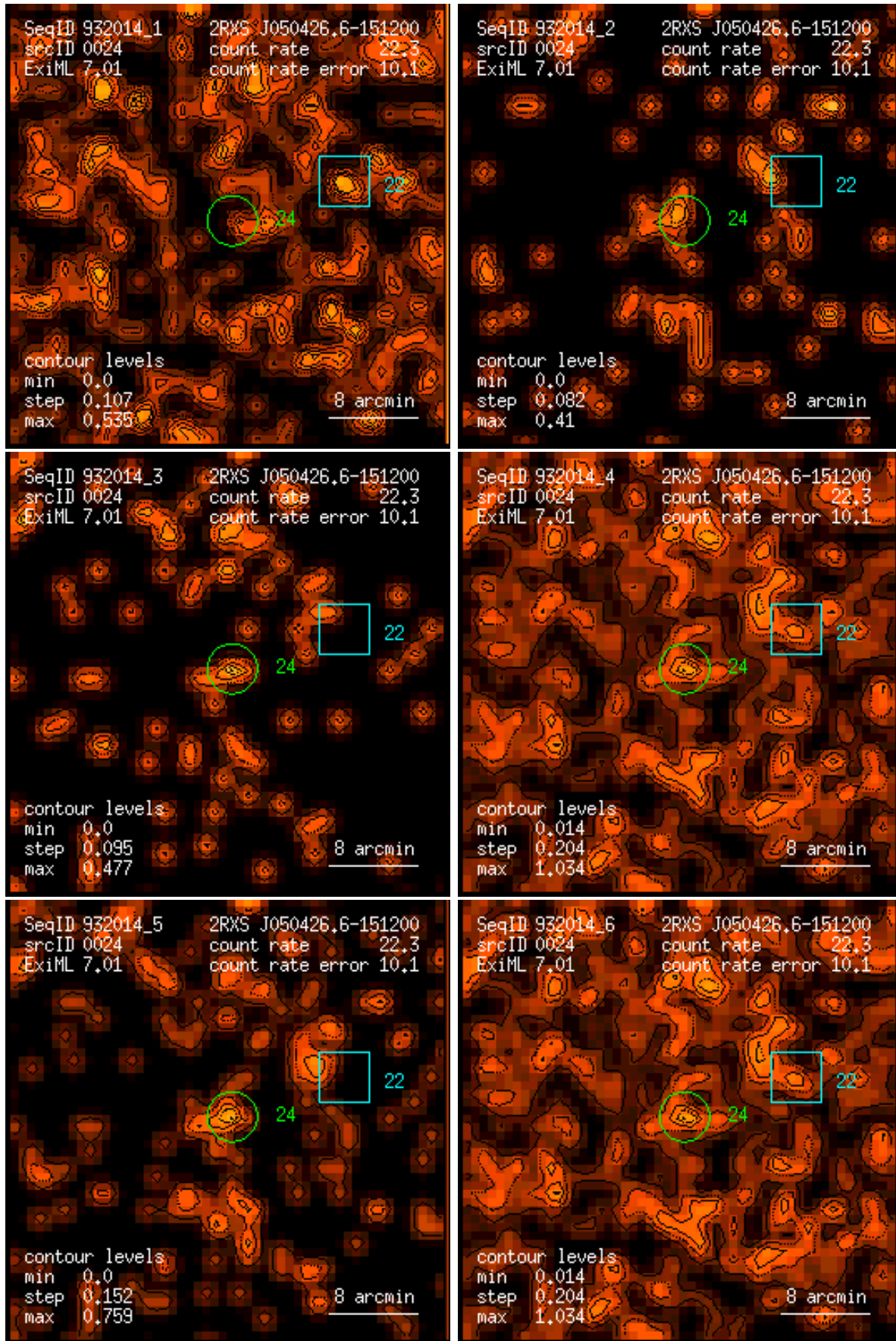
Figure 24: RASS 932014: detection 0024: band rate images, Gaussian filter: (1) PSPC channels 11 – 41, (2) 52 – 90, (3) 91 – 201, (4) 11 – 235, (5) 52 – 201, (6) 11 – 201. Broad band rates in counts/ks. Band rate contour levels in counts/ks/arcmin 2 .
