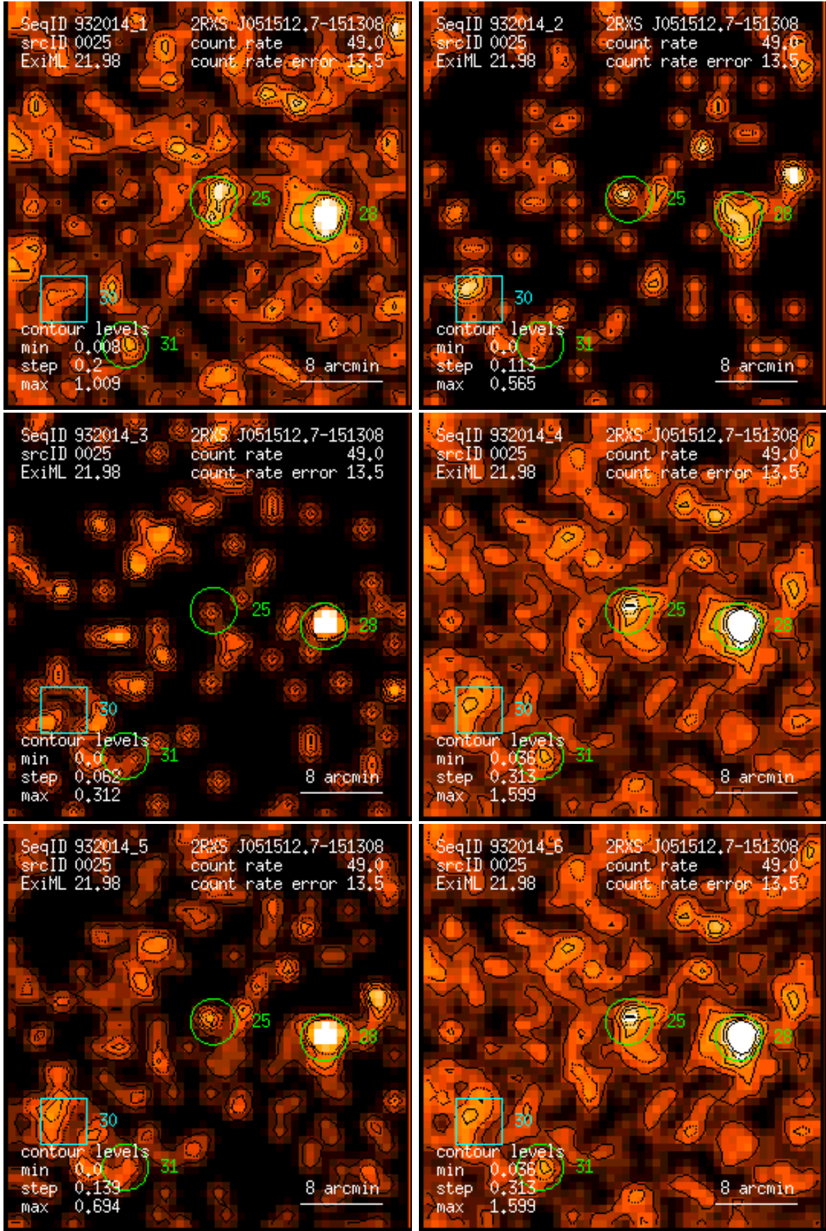
Figure 25: RASS 932014: detection 0025: band rate images, Gaussian filter: (1) PSPC channels 11 – 41, (2) 52 – 90, (3) 91 – 201, (4) 11 – 235, (5) 52 – 201, (6) 11 – 201. Broad band rates in counts/ks. Band rate contour levels in counts/ks/arcmin 2 .
