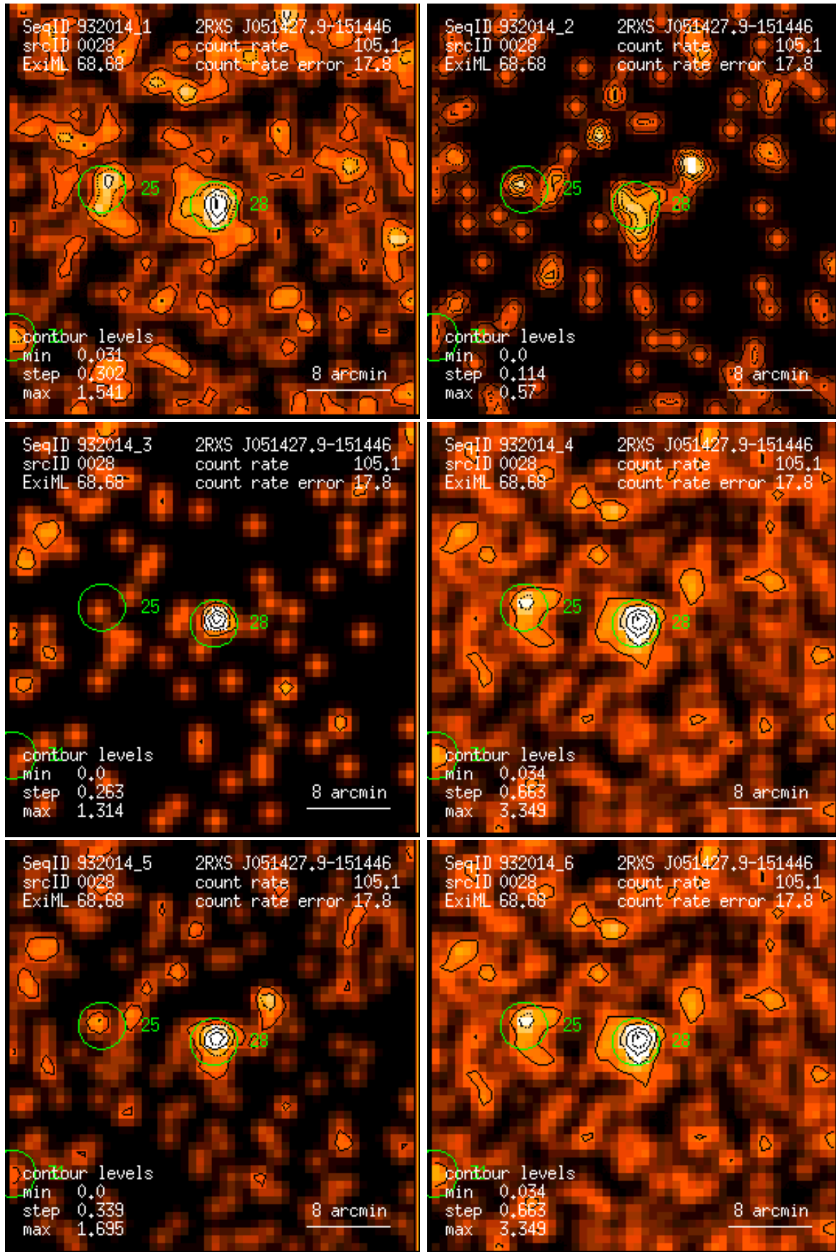
Figure 28: RASS 932014: detection 0028: band rate images, Gaussian filter: (1) PSPC channels 11 – 41, (2) 52 – 90, (3) 91 – 201, (4) 11 – 235, (5) 52 – 201, (6) 11 – 201. Broad band rates in counts/ks. Band rate contour levels in counts/ks/arcmin 2 .
