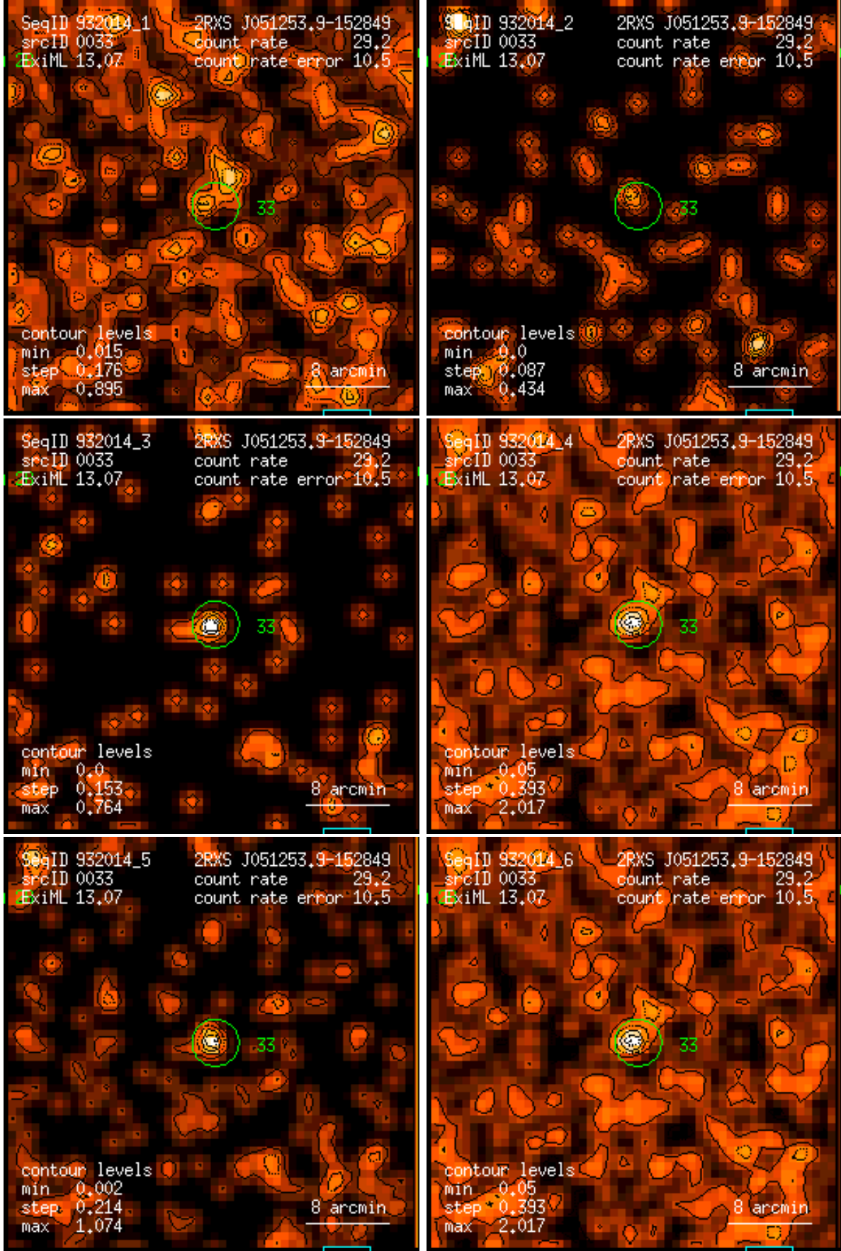
Figure 33: RASS 932014: detection 0033: band rate images, Gaussian filter: (1) PSPC channels 11 – 41, (2) 52 – 90, (3) 91 – 201, (4) 11 – 235, (5) 52 – 201, (6) 11 – 201. Broad band rates in counts/ks. Band rate contour levels in counts/ks/arcmin 2 .
