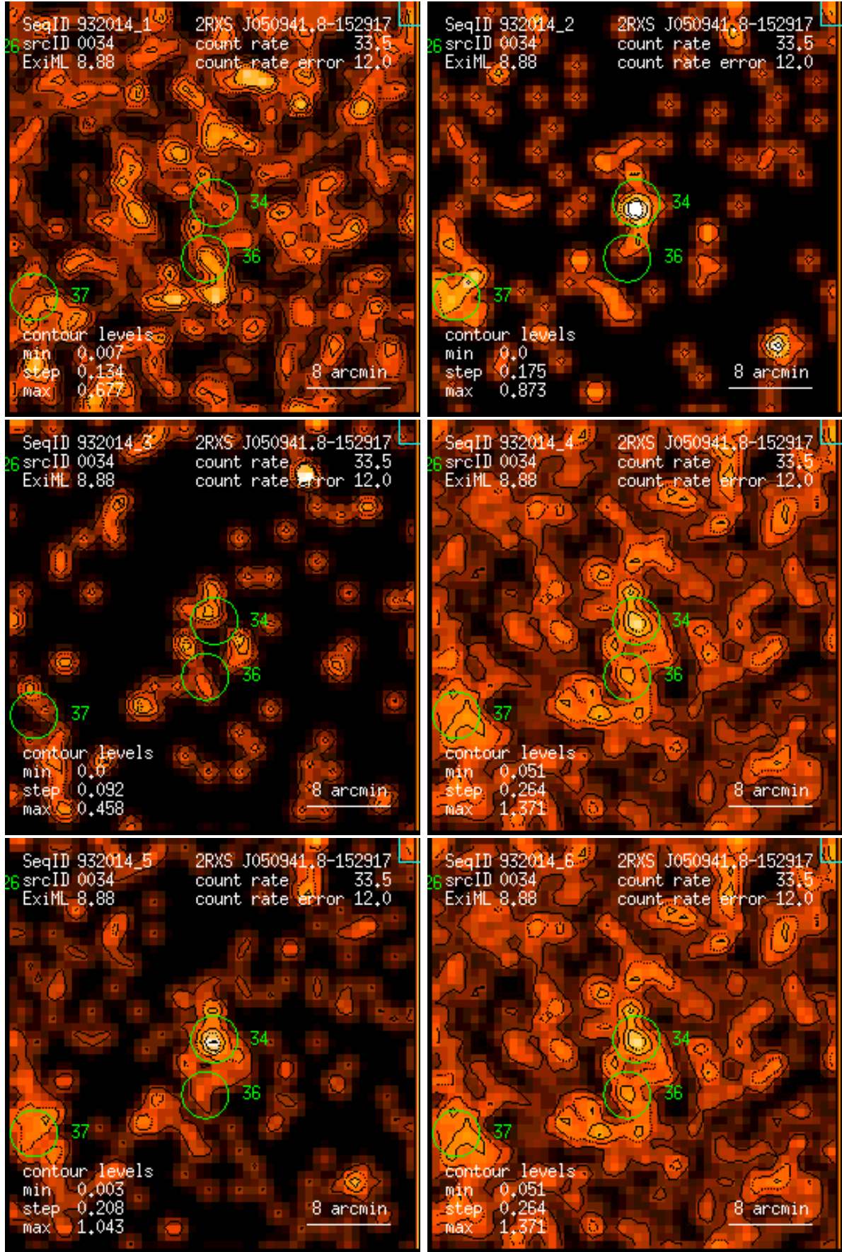
Figure 34: RASS 932014: detection 0034: band rate images, Gaussian filter: (1) PSPC channels 11 – 41, (2) 52 – 90, (3) 91 – 201, (4) 11 – 235, (5) 52 – 201, (6) 11 – 201. Broad band rates in counts/ks. Band rate contour levels in counts/ks/arcmin 2 .
