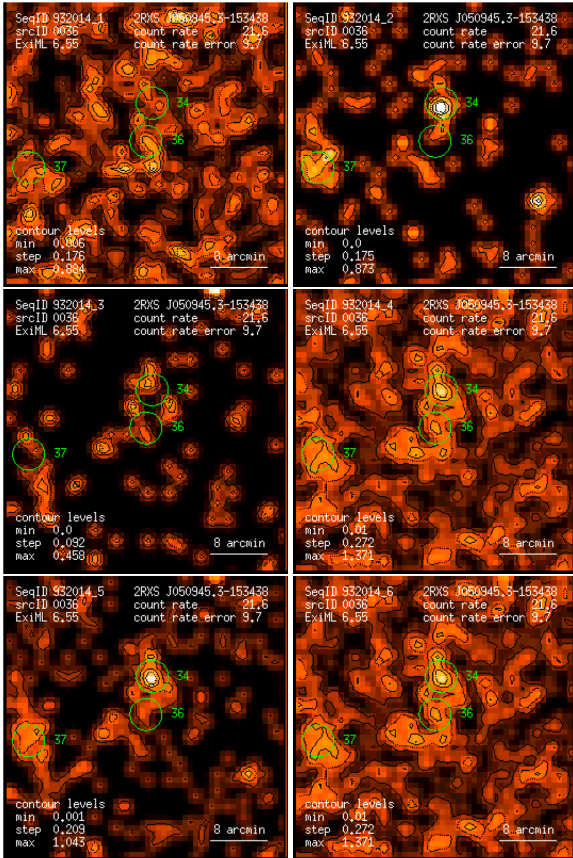
Figure 36: RASS 932014: detection 0036: band rate images, Gaussian filter: (1) PSPC channels 11 – 41, (2) 52 – 90, (3) 91 – 201, (4) 11 – 235, (5) 52 – 201, (6) 11 – 201. Broad band rates in counts/ks. Band rate contour levels in counts/ks/arcmin 2 .
