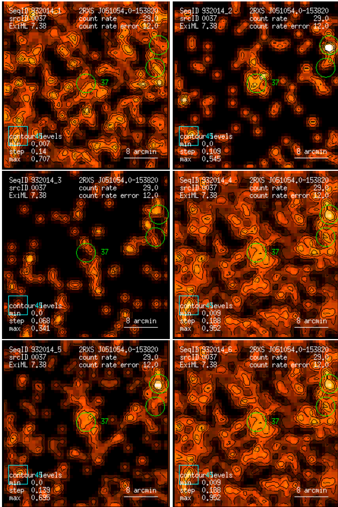
Figure 37: RASS 932014: detection 0037: band rate images, Gaussian filter: (1) PSPC channels 11 – 41, (2) 52 – 90, (3) 91 – 201, (4) 11 – 235, (5) 52 – 201, (6) 11 – 201. Broad band rates in counts/ks. Band rate contour levels in counts/ks/arcmin 2 .
