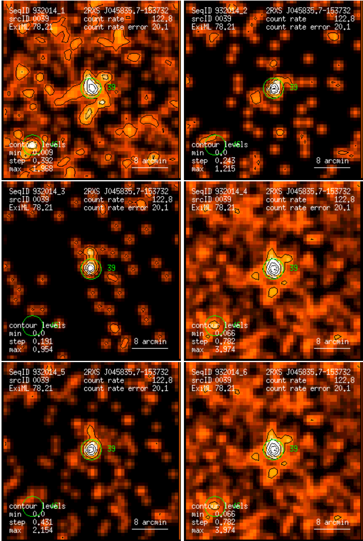
Figure 39: RASS 932014: detection 0039: band rate images, Gaussian filter: (1) PSPC channels 11 – 41, (2) 52 – 90, (3) 91 – 201, (4) 11 – 235, (5) 52 – 201, (6) 11 – 201. Broad band rates in counts/ks. Band rate contour levels in counts/ks/arcmin 2 .
