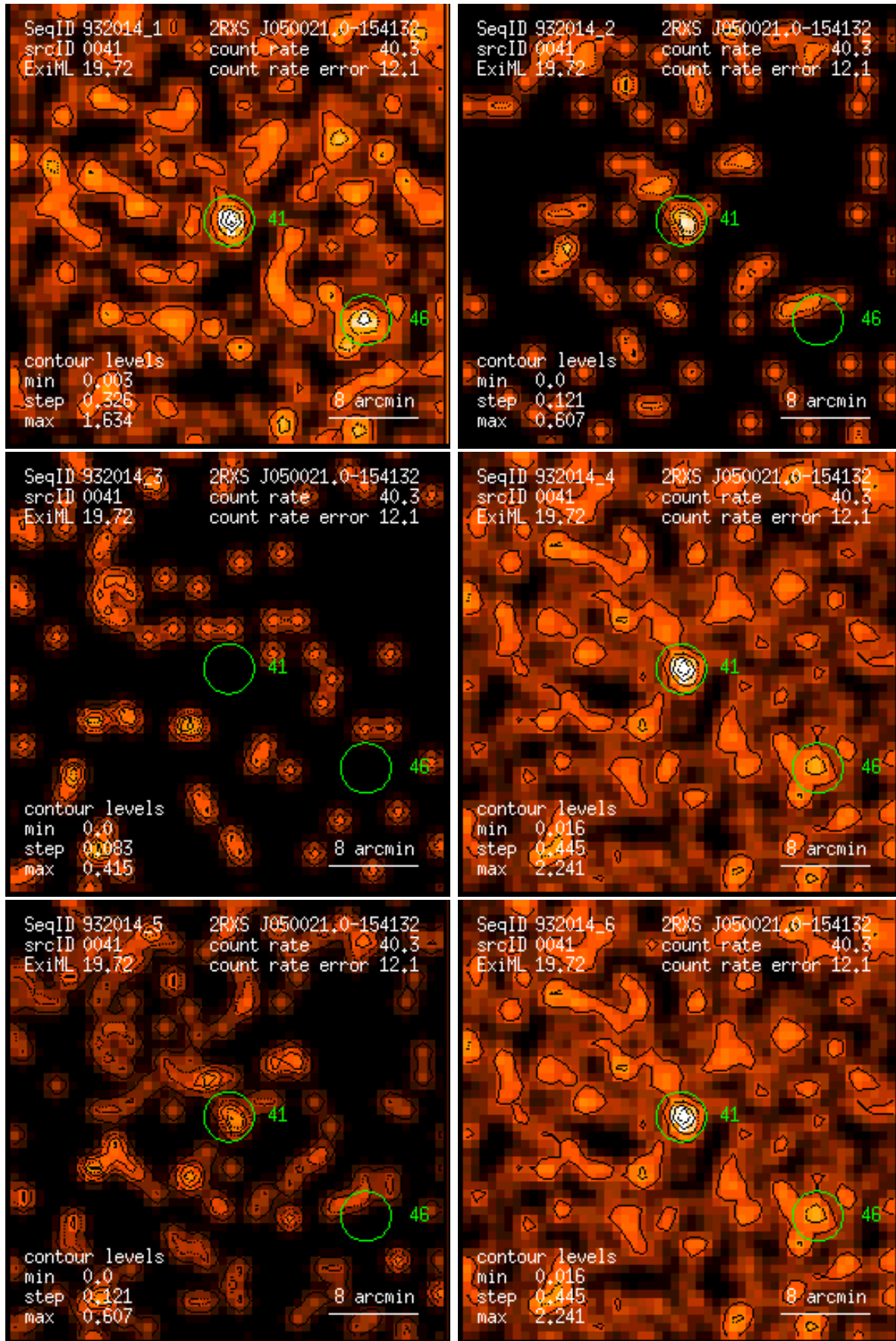
Figure 41: RASS 932014: detection 0041: band rate images, Gaussian filter: (1) PSPC channels 11 – 41, (2) 52 – 90, (3) 91 – 201, (4) 11 – 235, (5) 52 – 201, (6) 11 – 201. Broad band rates in counts/ks. Band rate contour levels in counts/ks/arcmin 2 .
