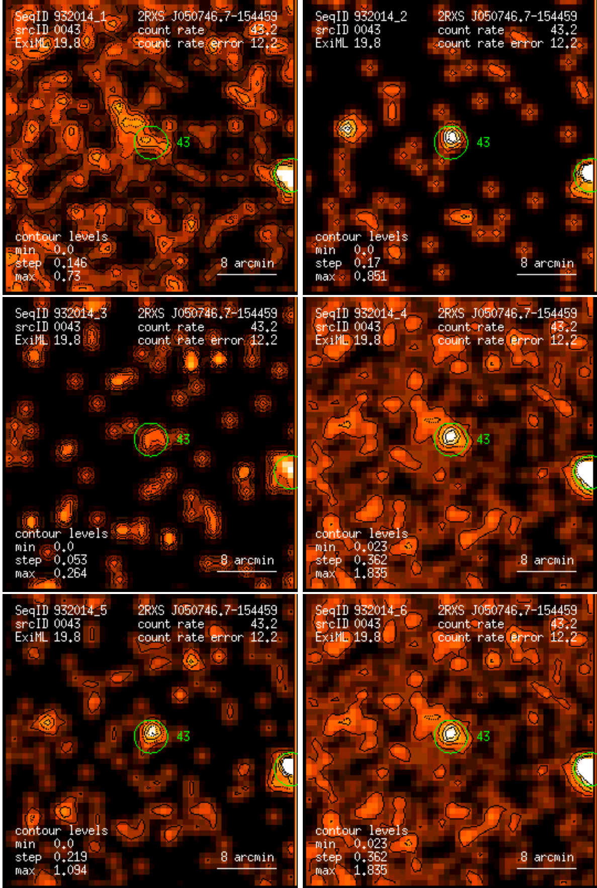
Figure 43: RASS 932014: detection 0043: band rate images, Gaussian filter: (1) PSPC channels 11 – 41, (2) 52 – 90, (3) 91 – 201, (4) 11 – 235, (5) 52 – 201, (6) 11 – 201. Broad band rates in counts/ks. Band rate contour levels in counts/ks/arcmin 2 .
