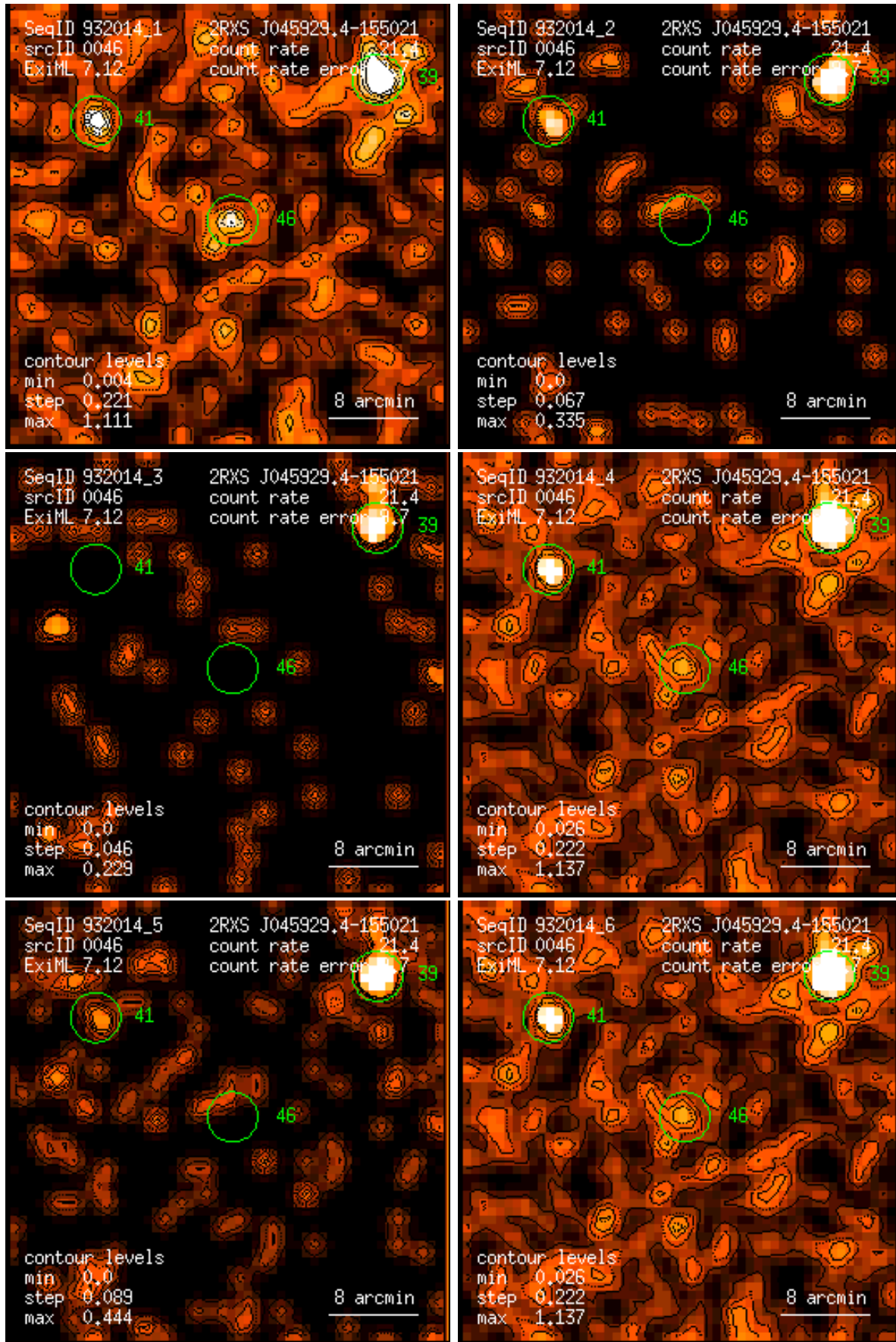
Figure 46: RASS 932014: detection 0046: band rate images, Gaussian filter: (1) PSPC channels 11 – 41, (2) 52 – 90, (3) 91 – 201, (4) 11 – 235, (5) 52 – 201, (6) 11 – 201. Broad band rates in counts/ks. Band rate contour levels in counts/ks/arcmin 2 .
