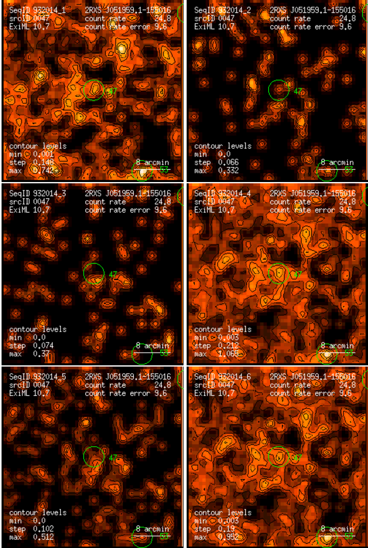
Figure 47: RASS 932014: detection 0047: band rate images, Gaussian filter: (1) PSPC channels 11 – 41, (2) 52 – 90, (3) 91 – 201, (4) 11 – 235, (5) 52 – 201, (6) 11 – 201. Broad band rates in counts/ks. Band rate contour levels in counts/ks/arcmin 2 .
