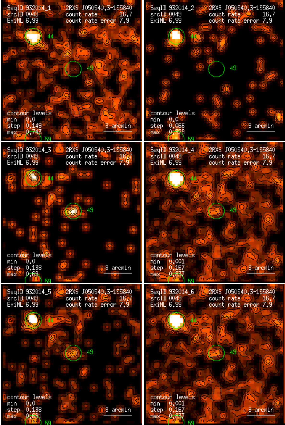
Figure 49: RASS 932014: detection 0049: band rate images, Gaussian filter: (1) PSPC channels 11 – 41, (2) 52 – 90, (3) 91 – 201, (4) 11 – 235, (5) 52 – 201, (6) 11 – 201. Broad band rates in counts/ks. Band rate contour levels in counts/ks/arcmin 2 .
