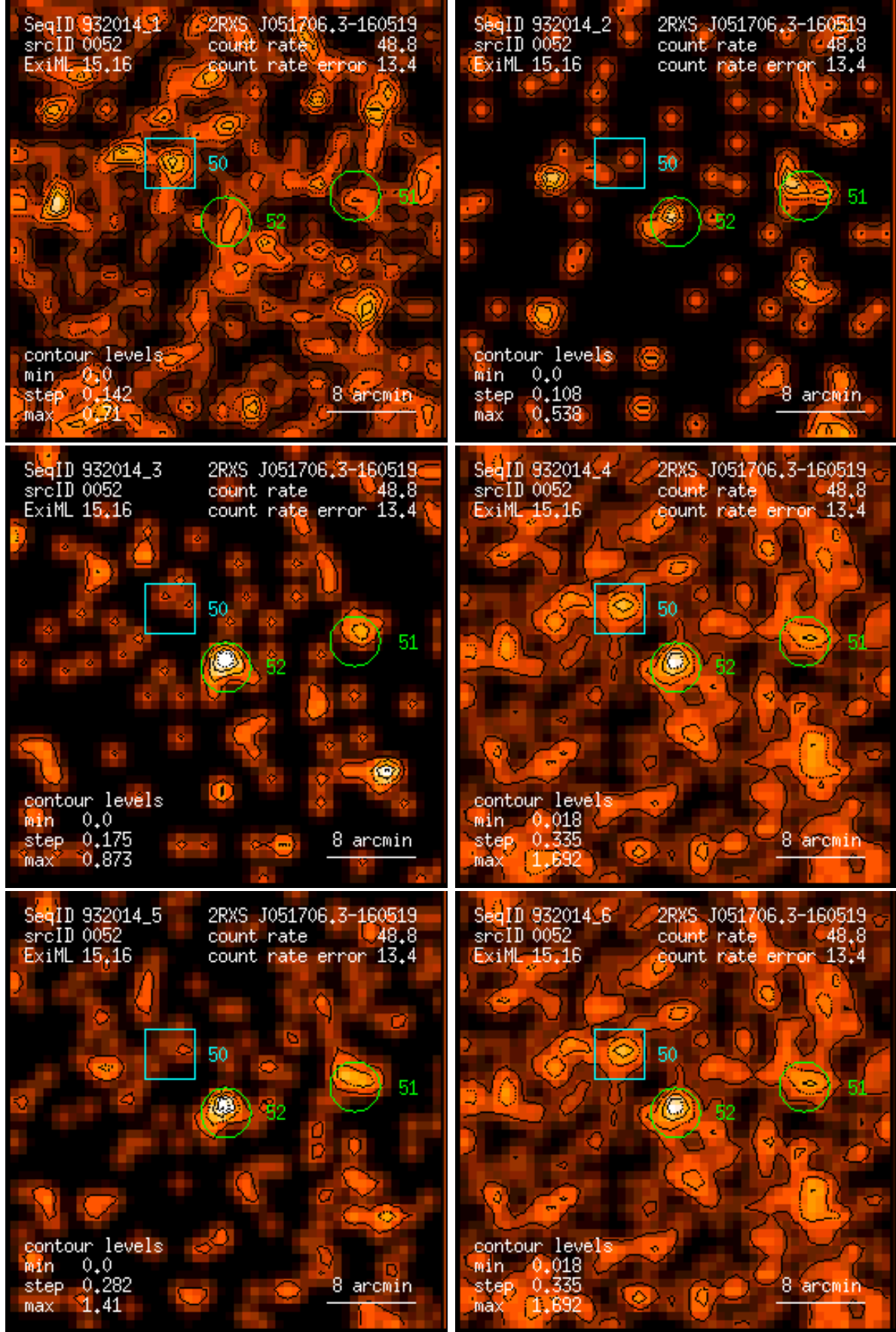
Figure 52: RASS 932014: detection 0052: band rate images, Gaussian filter: (1) PSPC channels 11 – 41, (2) 52 – 90, (3) 91 – 201, (4) 11 – 235, (5) 52 – 201, (6) 11 – 201. Broad band rates in counts/ks. Band rate contour levels in counts/ks/arcmin 2 .
