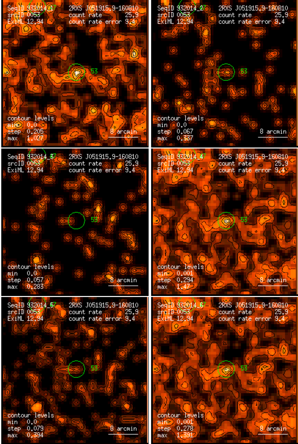
Figure 53: RASS 932014: detection 0053: band rate images, Gaussian filter: (1) PSPC channels 11 – 41, (2) 52 – 90, (3) 91 – 201, (4) 11 – 235, (5) 52 – 201, (6) 11 – 201. Broad band rates in counts/ks. Band rate contour levels in counts/ks/arcmin 2 .
