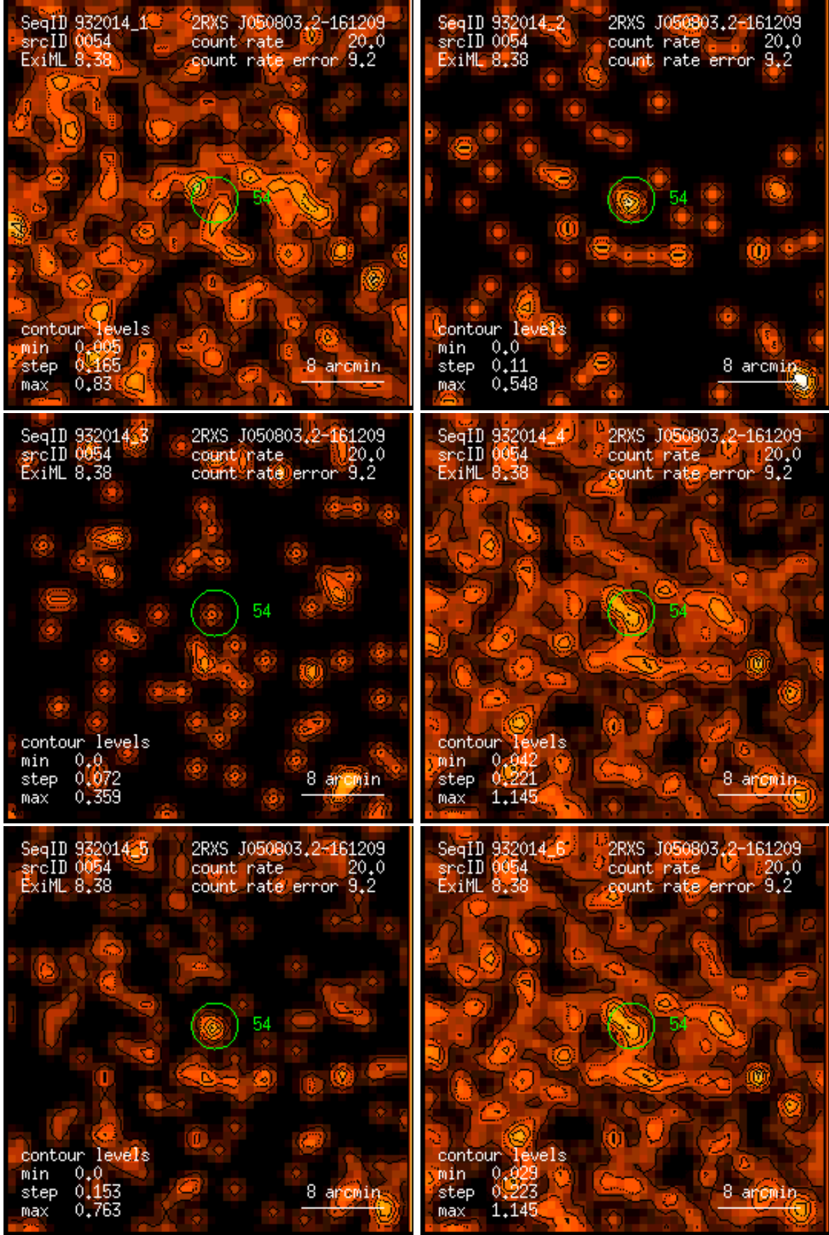
Figure 54: RASS 932014: detection 0054: band rate images, Gaussian filter: (1) PSPC channels 11 – 41, (2) 52 – 90, (3) 91 – 201, (4) 11 – 235, (5) 52 – 201, (6) 11 – 201. Broad band rates in counts/ks. Band rate contour levels in counts/ks/arcmin 2 .
