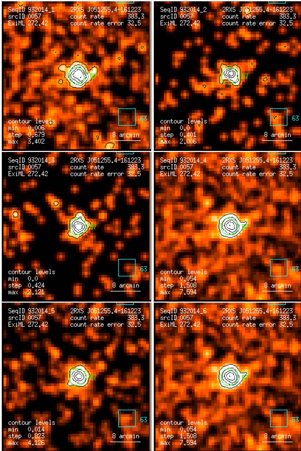
Figure 57: RASS 932014: detection 0057: band rate images, Gaussian filter: (1) PSPC channels 11 – 41, (2) 52 – 90, (3) 91 – 201, (4) 11 – 235, (5) 52 – 201, (6) 11 – 201. Broad band rates in counts/ks. Band rate contour levels in counts/ks/arcmin 2 .
