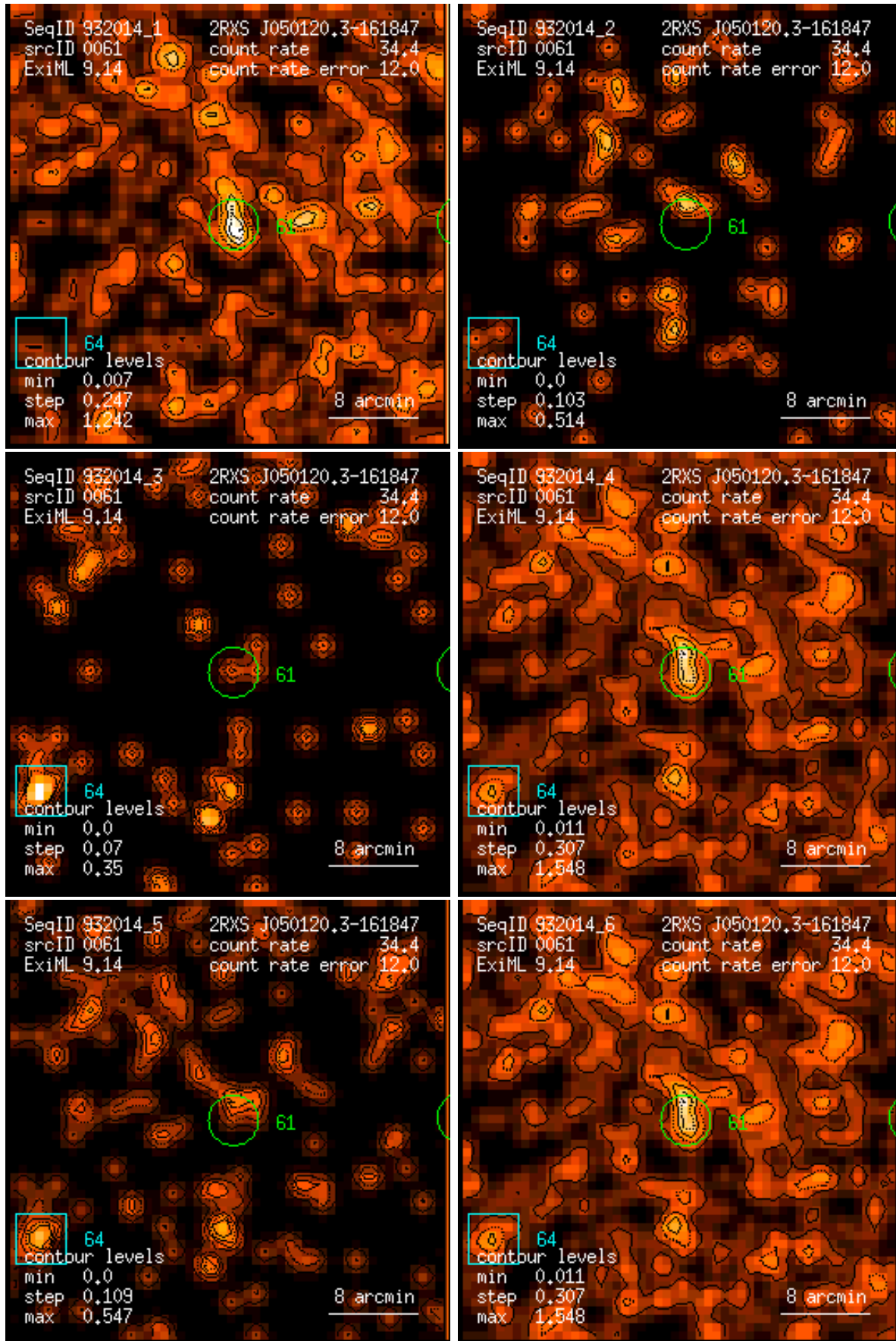
Figure 61: RASS 932014: detection 0061: band rate images, Gaussian filter: (1) PSPC channels 11 – 41, (2) 52 – 90, (3) 91 – 201, (4) 11 – 235, (5) 52 – 201, (6) 11 – 201. Broad band rates in counts/ks. Band rate contour levels in counts/ks/arcmin 2 .
