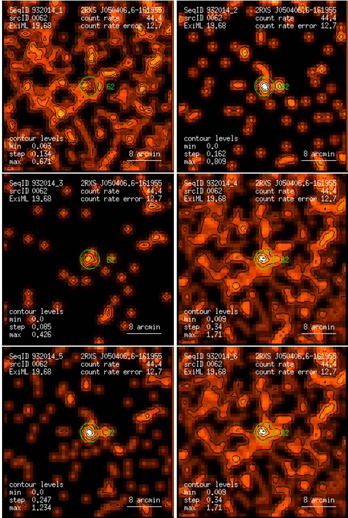
Figure 62: RASS 932014: detection 0062: band rate images, Gaussian filter: (1) PSPC channels 11 – 41, (2) 52 – 90, (3) 91 – 201, (4) 11 – 235, (5) 52 – 201, (6) 11 – 201. Broad band rates in counts/ks. Band rate contour levels in counts/ks/arcmin 2 .
