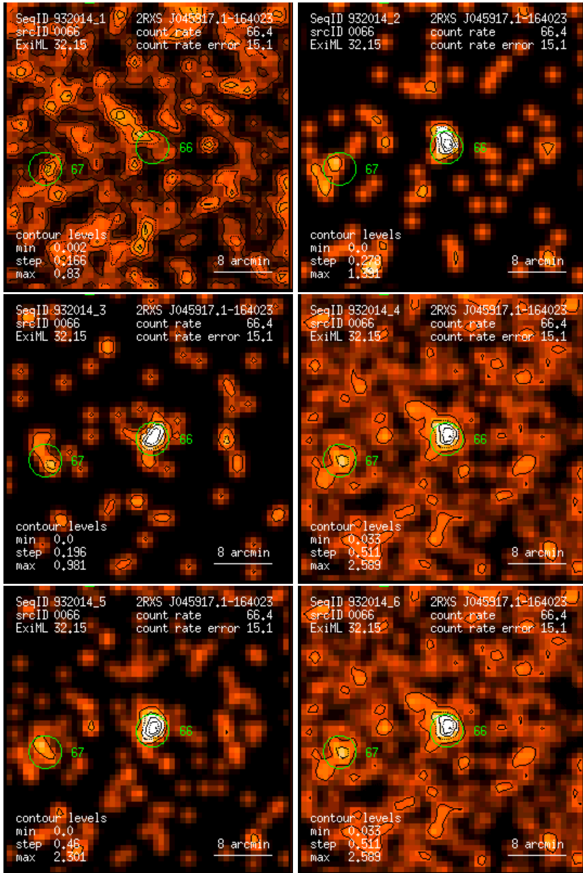
Figure 66: RASS 932014: detection 0066: band rate images, Gaussian filter: (1) PSPC channels 11 – 41, (2) 52 – 90, (3) 91 – 201, (4) 11 – 235, (5) 52 – 201, (6) 11 – 201. Broad band rates in counts/ks. Band rate contour levels in counts/ks/arcmin 2 .
