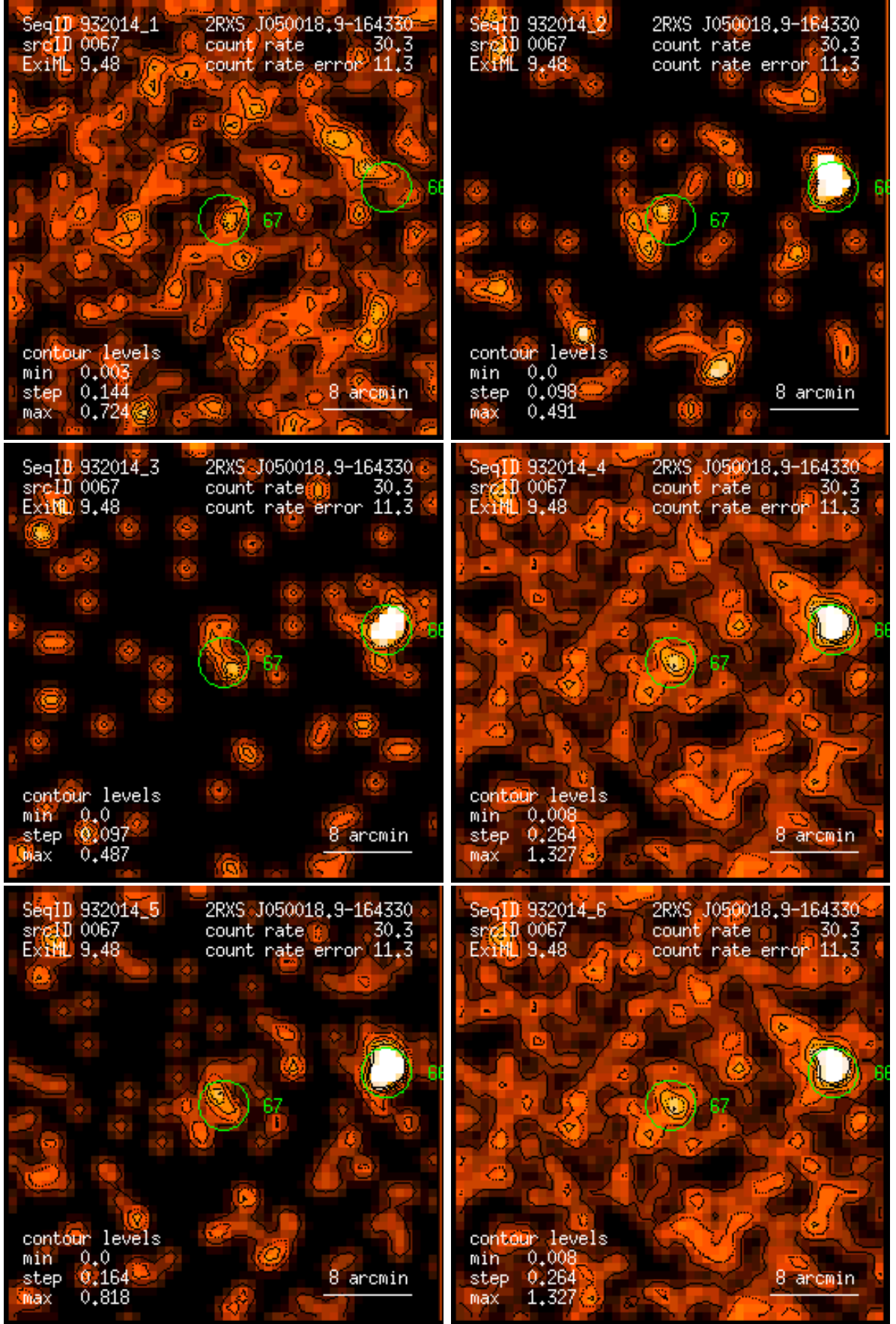
Figure 67: RASS 932014: detection 0067: band rate images, Gaussian filter: (1) PSPC channels 11 – 41, (2) 52 – 90, (3) 91 – 201, (4) 11 – 235, (5) 52 – 201, (6) 11 – 201. Broad band rates in counts/ks. Band rate contour levels in counts/ks/arcmin 2 .
