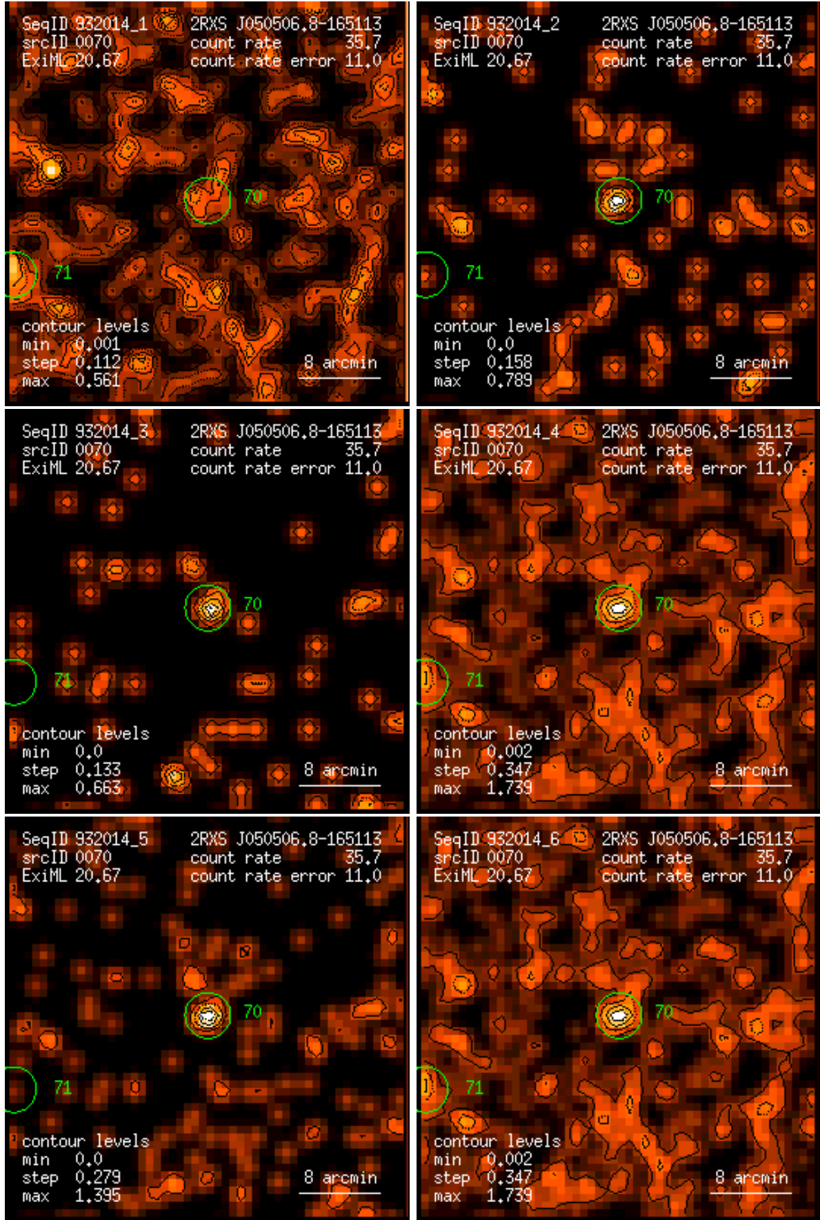
Figure 70: RASS 932014: detection 0070: band rate images, Gaussian filter: (1) PSPC channels 11 – 41, (2) 52 – 90, (3) 91 – 201, (4) 11 – 235, (5) 52 – 201, (6) 11 – 201. Broad band rates in counts/ks. Band rate contour levels in counts/ks/arcmin 2 .
