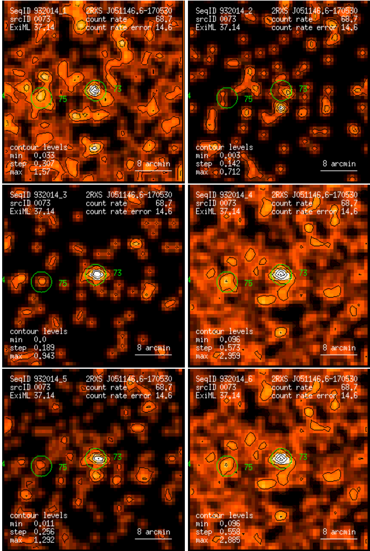
Figure 73: RASS 932014: detection 0073: band rate images, Gaussian filter: (1) PSPC channels 11 – 41, (2) 52 – 90, (3) 91 – 201, (4) 11 – 235, (5) 52 – 201, (6) 11 – 201. Broad band rates in counts/ks. Band rate contour levels in counts/ks/arcmin 2 .
