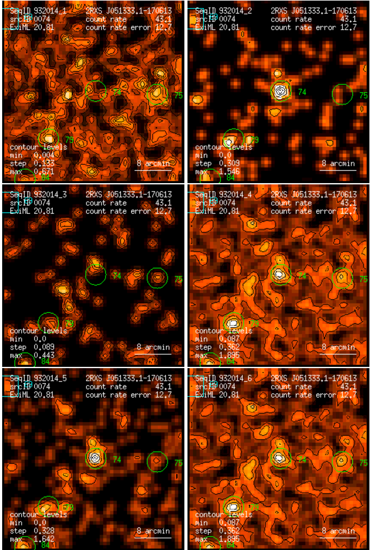
Figure 74: RASS 932014: detection 0074: band rate images, Gaussian filter: (1) PSPC channels 11 – 41, (2) 52 – 90, (3) 91 – 201, (4) 11 – 235, (5) 52 – 201, (6) 11 – 201. Broad band rates in counts/ks. Band rate contour levels in counts/ks/arcmin 2 .
