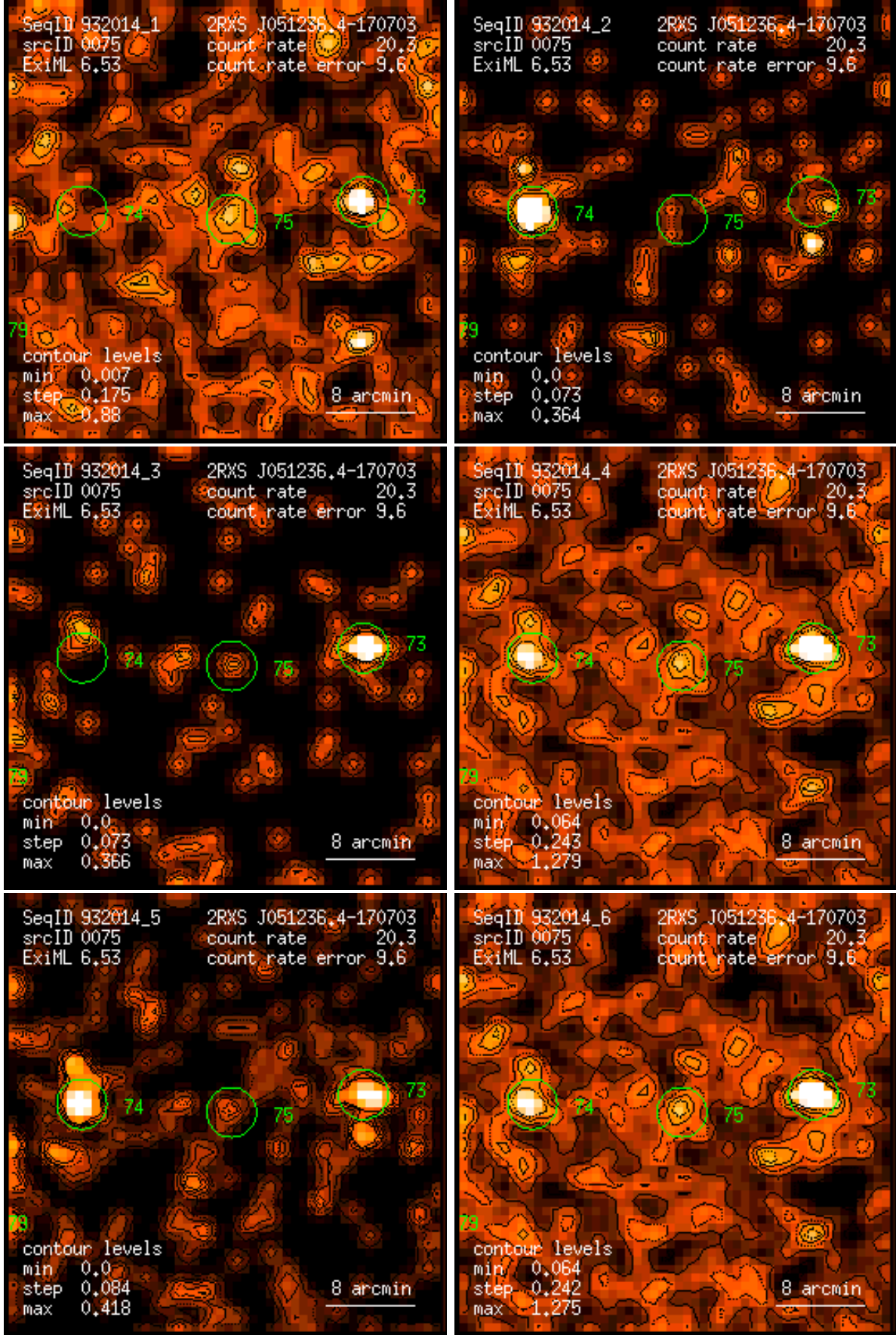
Figure 75: RASS 932014: detection 0075: band rate images, Gaussian filter: (1) PSPC channels 11 – 41, (2) 52 – 90, (3) 91 – 201, (4) 11 – 235, (5) 52 – 201, (6) 11 – 201. Broad band rates in counts/ks. Band rate contour levels in counts/ks/arcmin 2 .
