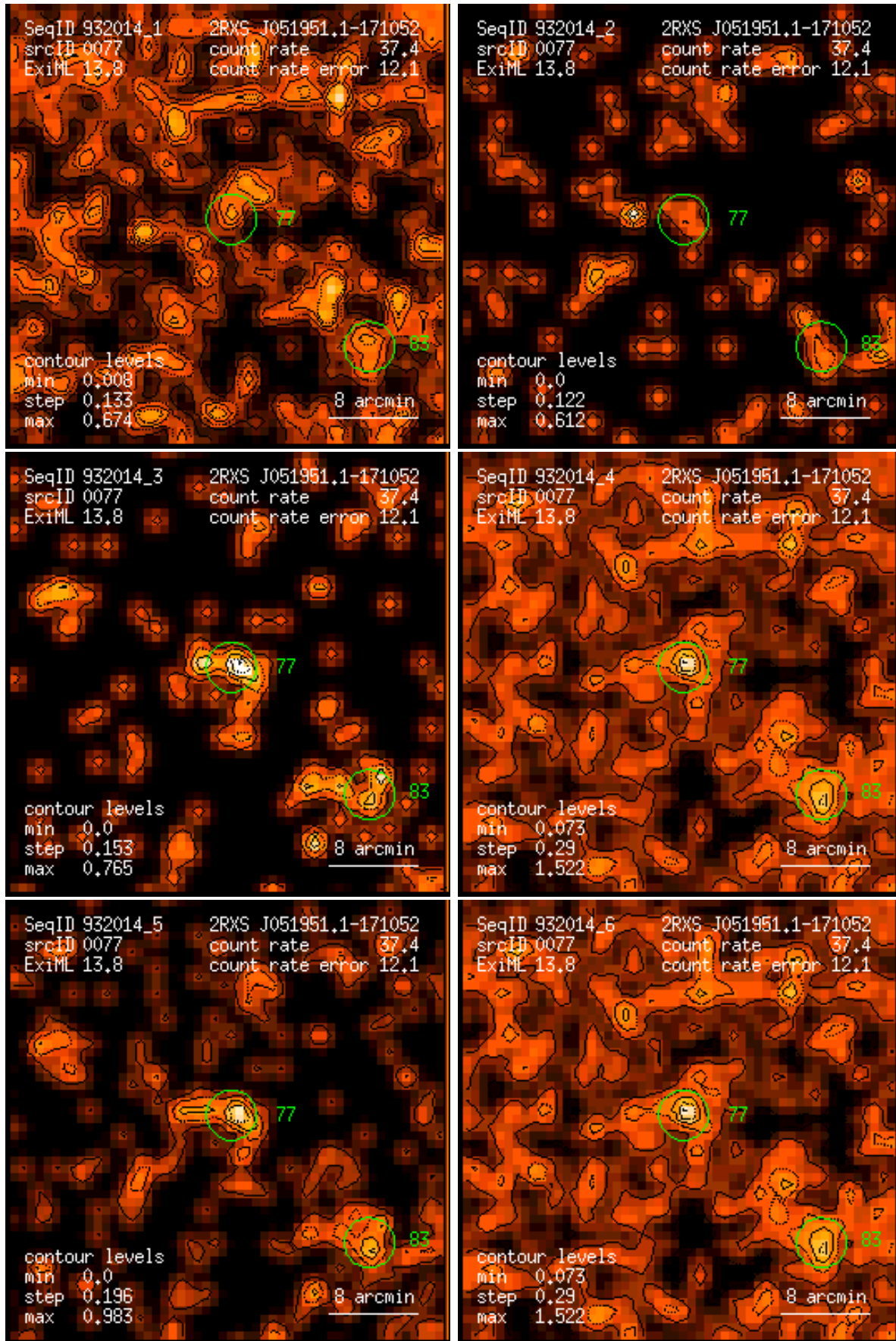
Figure 77: RASS 932014: detection 0077: band rate images, Gaussian filter: (1) PSPC channels 11 – 41, (2) 52 – 90, (3) 91 – 201, (4) 11 – 235, (5) 52 – 201, (6) 11 – 201. Broad band rates in counts/ks. Band rate contour levels in counts/ks/arcmin 2 .
