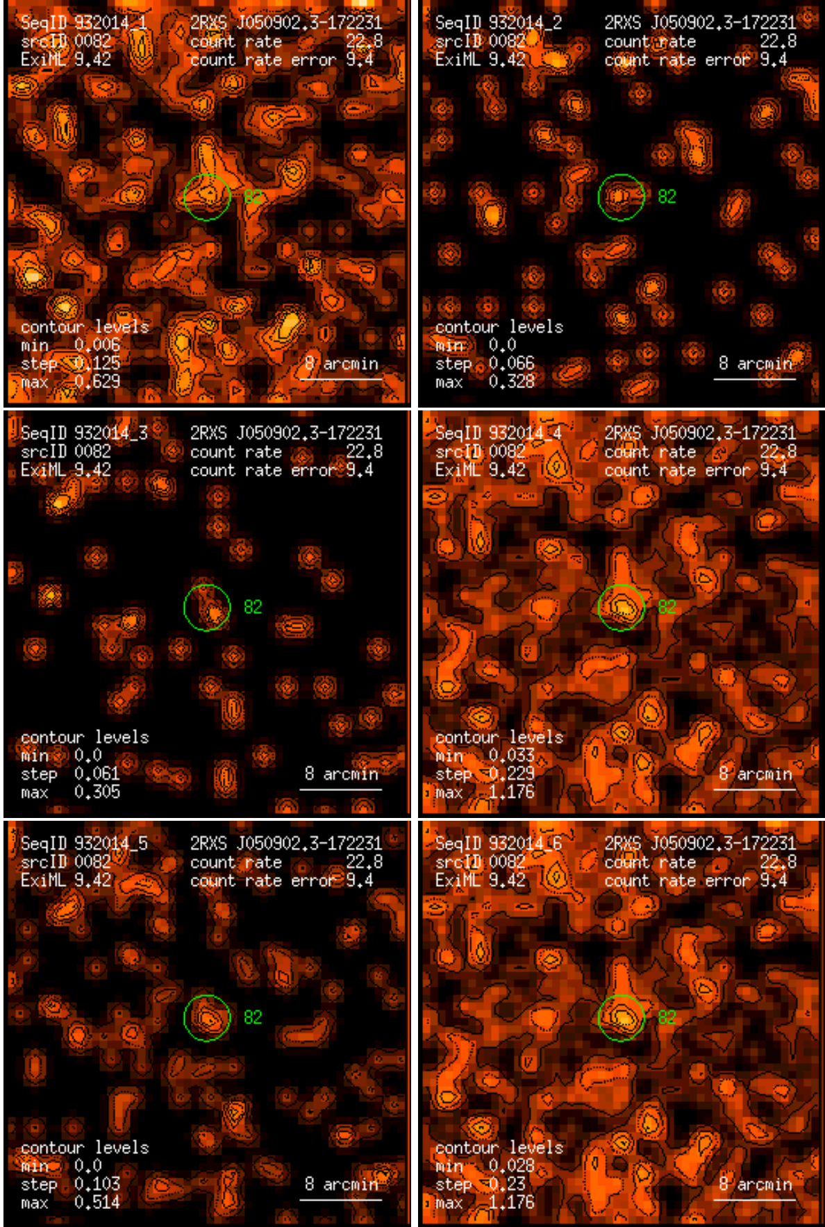
Figure 82: RASS 932014: detection 0082: band rate images, Gaussian filter: (1) PSPC channels 11 – 41, (2) 52 – 90, (3) 91 – 201, (4) 11 – 235, (5) 52 – 201, (6) 11 – 201. Broad band rates in counts/ks. Band rate contour levels in counts/ks/arcmin 2 .
