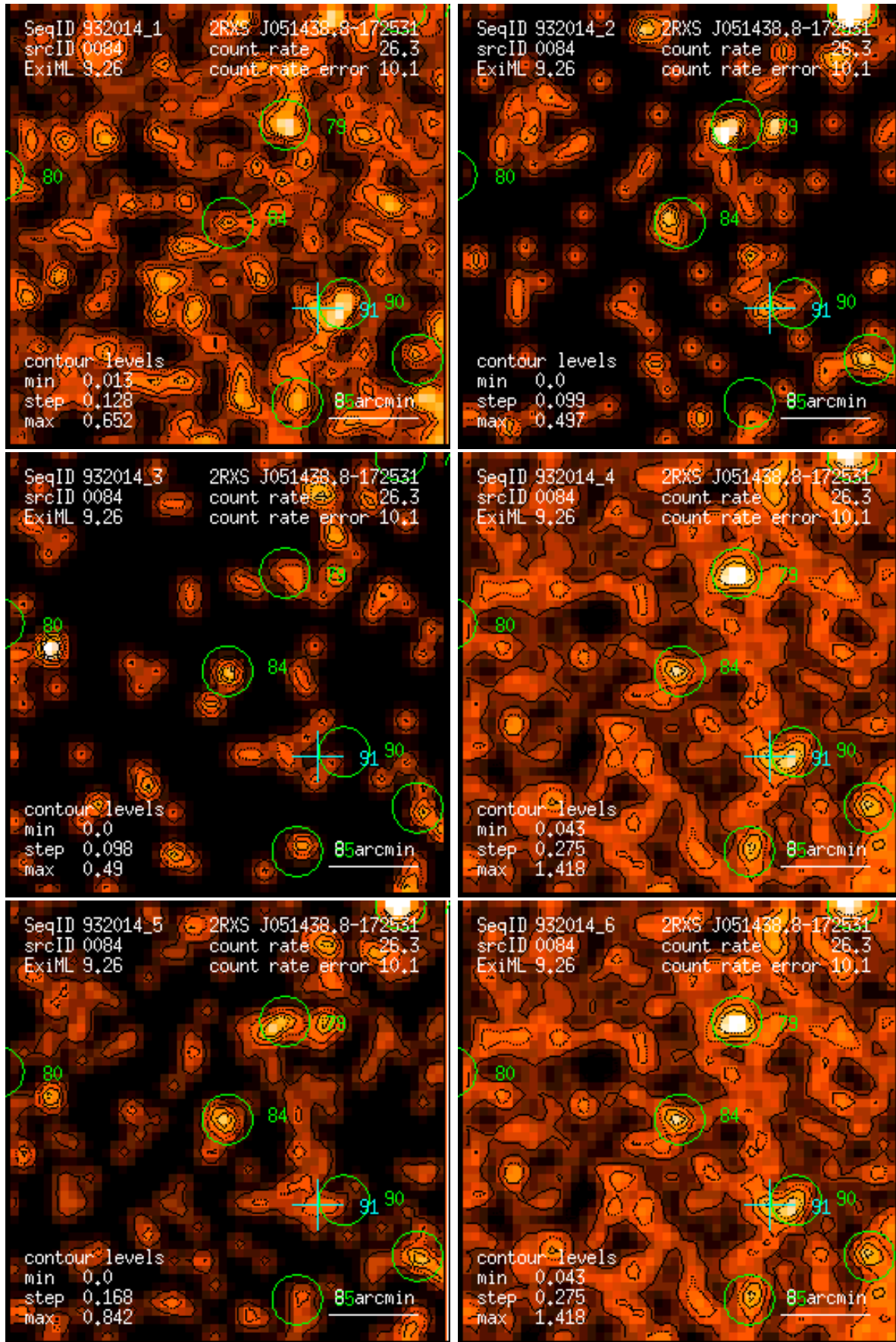
Figure 84: RASS 932014: detection 0084: band rate images, Gaussian filter: (1) PSPC channels 11 – 41, (2) 52 – 90, (3) 91 – 201, (4) 11 – 235, (5) 52 – 201, (6) 11 – 201. Broad band rates in counts/ks. Band rate contour levels in counts/ks/arcmin 2 .
