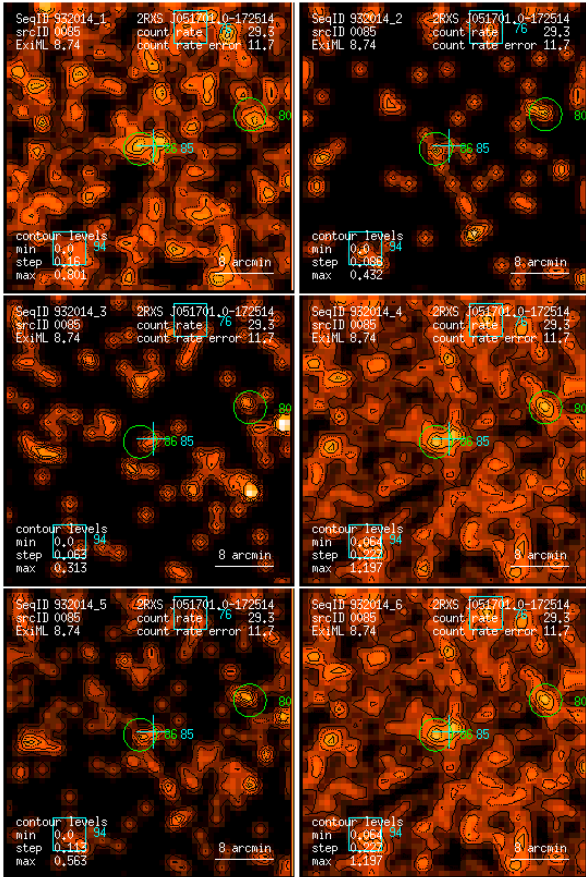
Figure 85: RASS 932014: detection 0085: band rate images, Gaussian filter: (1) PSPC channels 11 – 41, (2) 52 – 90, (3) 91 – 201, (4) 11 – 235, (5) 52 – 201, (6) 11 – 201. Broad band rates in counts/ks. Band rate contour levels in counts/ks/arcmin 2 .
