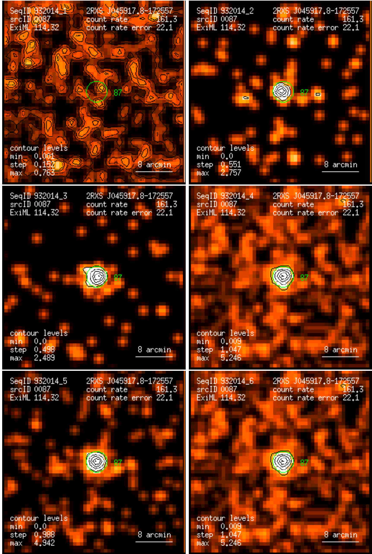
Figure 87: RASS 932014: detection 0087: band rate images, Gaussian filter: (1) PSPC channels 11 – 41, (2) 52 – 90, (3) 91 – 201, (4) 11 – 235, (5) 52 – 201, (6) 11 – 201. Broad band rates in counts/ks. Band rate contour levels in counts/ks/arcmin 2 .
