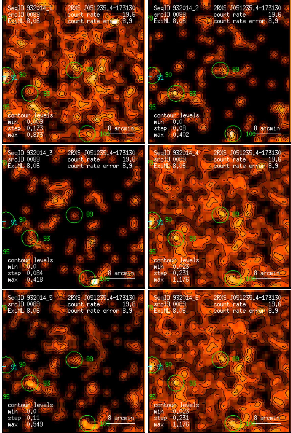
Figure 89: RASS 932014: detection 0089: band rate images, Gaussian filter: (1) PSPC channels 11 – 41, (2) 52 – 90, (3) 91 – 201, (4) 11 – 235, (5) 52 – 201, (6) 11 – 201. Broad band rates in counts/ks. Band rate contour levels in counts/ks/arcmin 2 .
