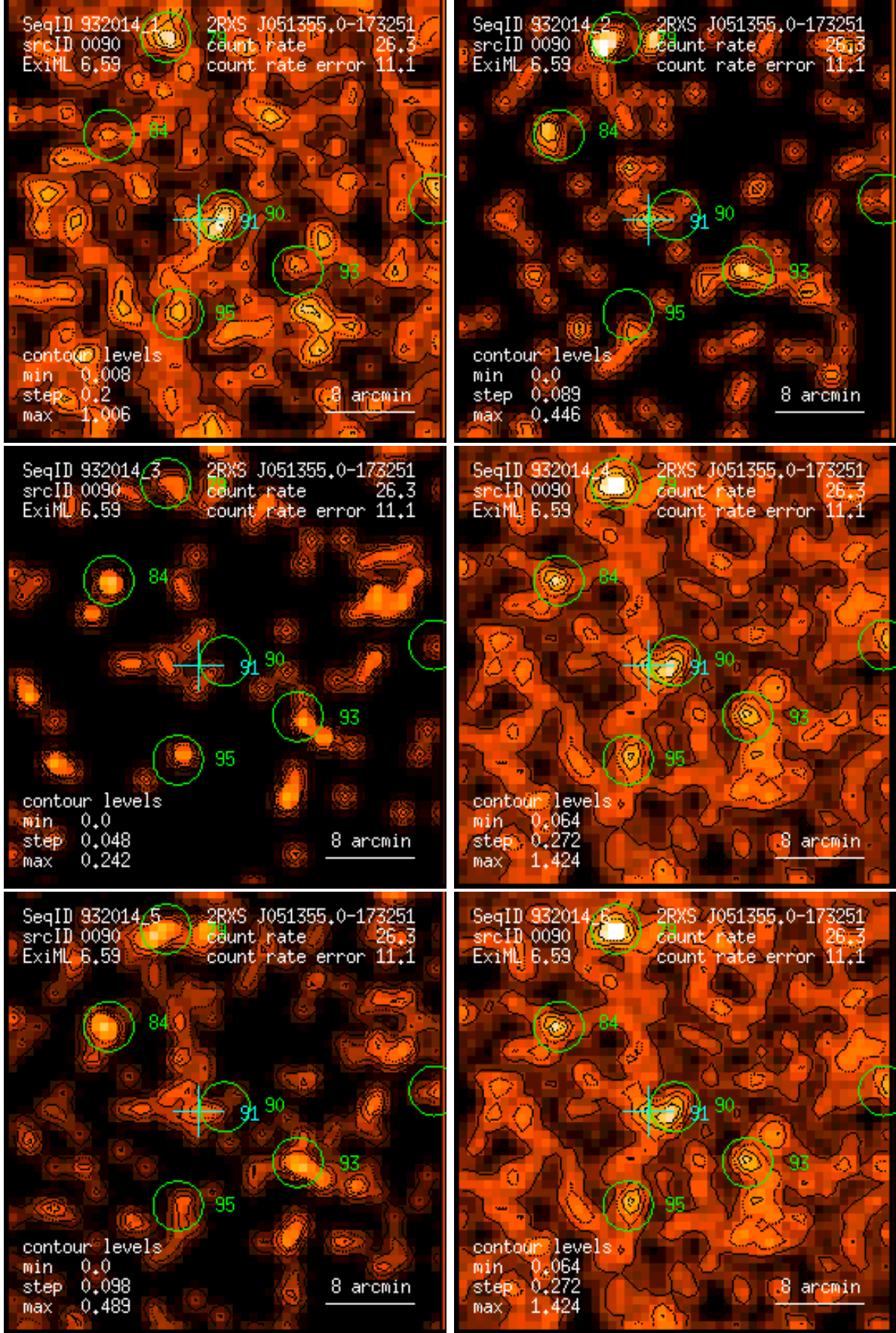
Figure 90: RASS 932014: detection 0090: band rate images, Gaussian filter: (1) PSPC channels 11 – 41, (2) 52 – 90, (3) 91 – 201, (4) 11 – 235, (5) 52 – 201, (6) 11 – 201. Broad band rates in counts/ks. Band rate contour levels in counts/ks/arcmin 2 .
