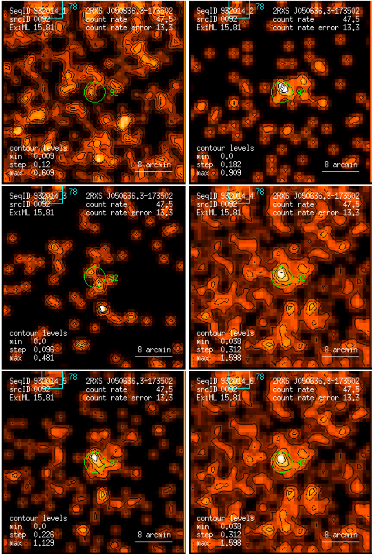
Figure 92: RASS 932014: detection 0092: band rate images, Gaussian filter: (1) PSPC channels 11 – 41, (2) 52 – 90, (3) 91 – 201, (4) 11 – 235, (5) 52 – 201, (6) 11 – 201. Broad band rates in counts/ks. Band rate contour levels in counts/ks/arcmin 2 .
