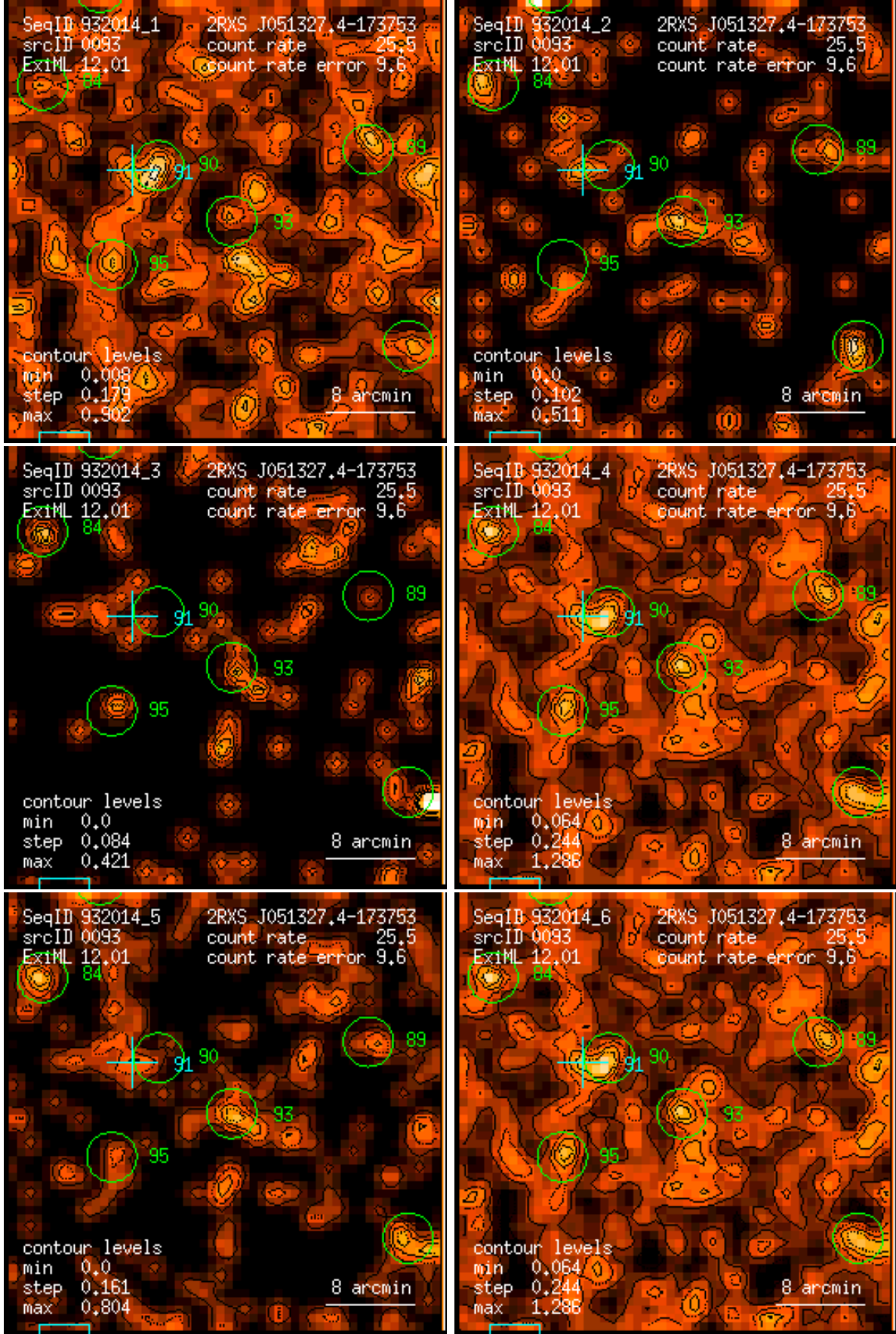
Figure 93: RASS 932014: detection 0093: band rate images, Gaussian filter: (1) PSPC channels 11 – 41, (2) 52 – 90, (3) 91 – 201, (4) 11 – 235, (5) 52 – 201, (6) 11 – 201. Broad band rates in counts/ks. Band rate contour levels in counts/ks/arcmin 2 .
