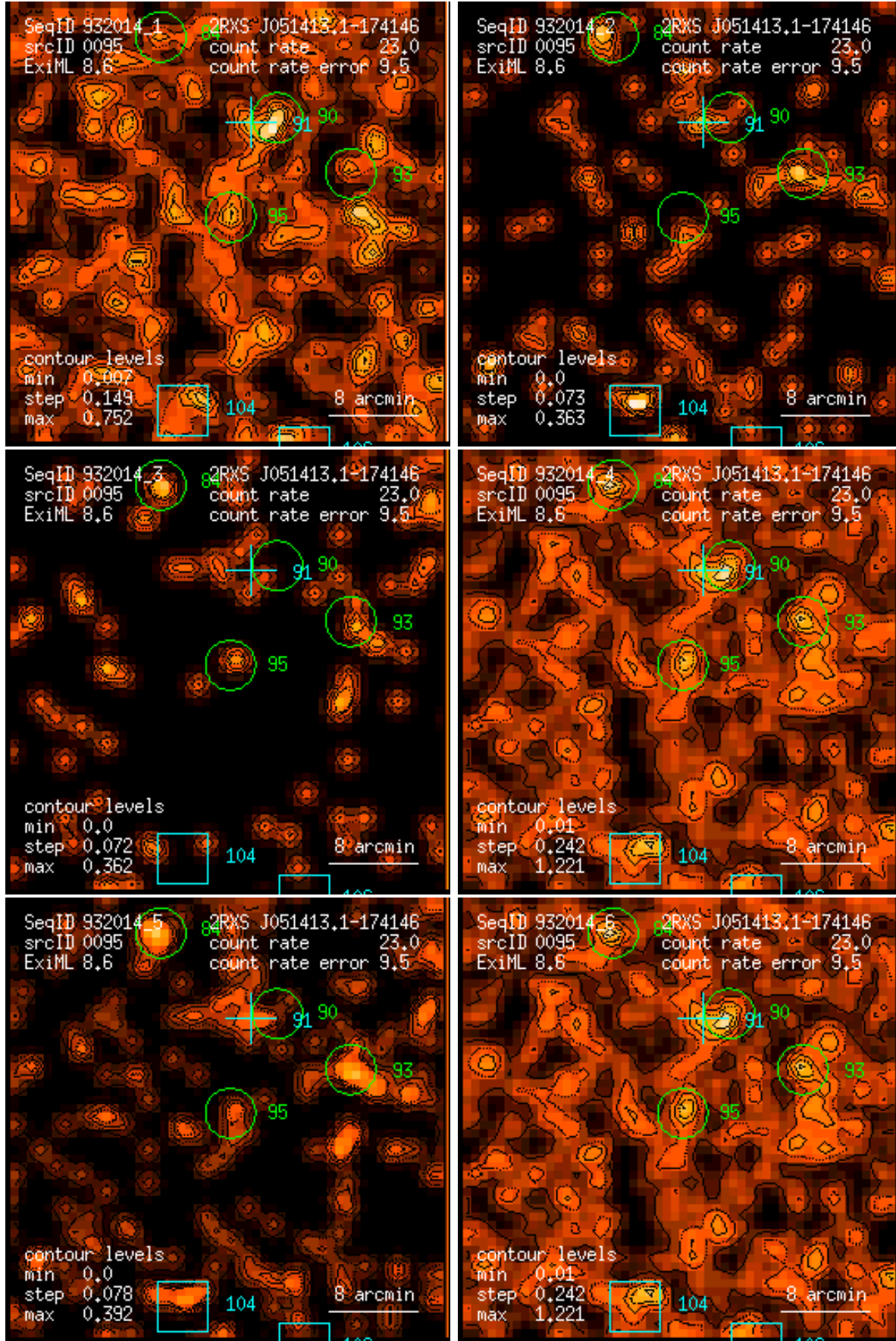
Figure 95: RASS 932014: detection 0095: band rate images, Gaussian filter: (1) PSPC channels 11 – 41, (2) 52 – 90, (3) 91 – 201, (4) 11 – 235, (5) 52 – 201, (6) 11 – 201. Broad band rates in counts/ks. Band rate contour levels in counts/ks/arcmin 2 .
