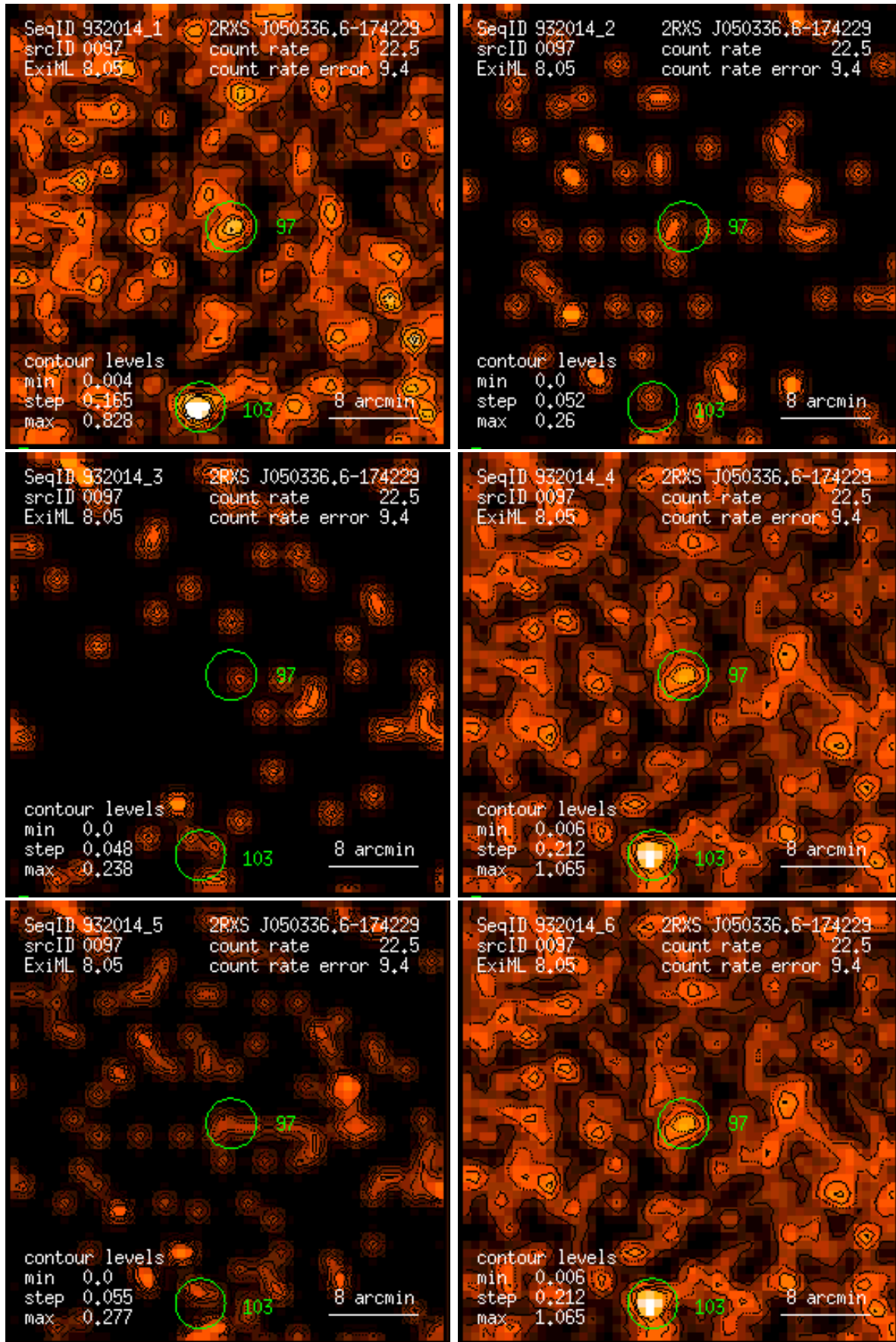
Figure 97: RASS 932014: detection 0097: band rate images, Gaussian filter: (1) PSPC channels 11 – 41, (2) 52 – 90, (3) 91 – 201, (4) 11 – 235, (5) 52 – 201, (6) 11 – 201. Broad band rates in counts/ks. Band rate contour levels in counts/ks/arcmin 2 .
