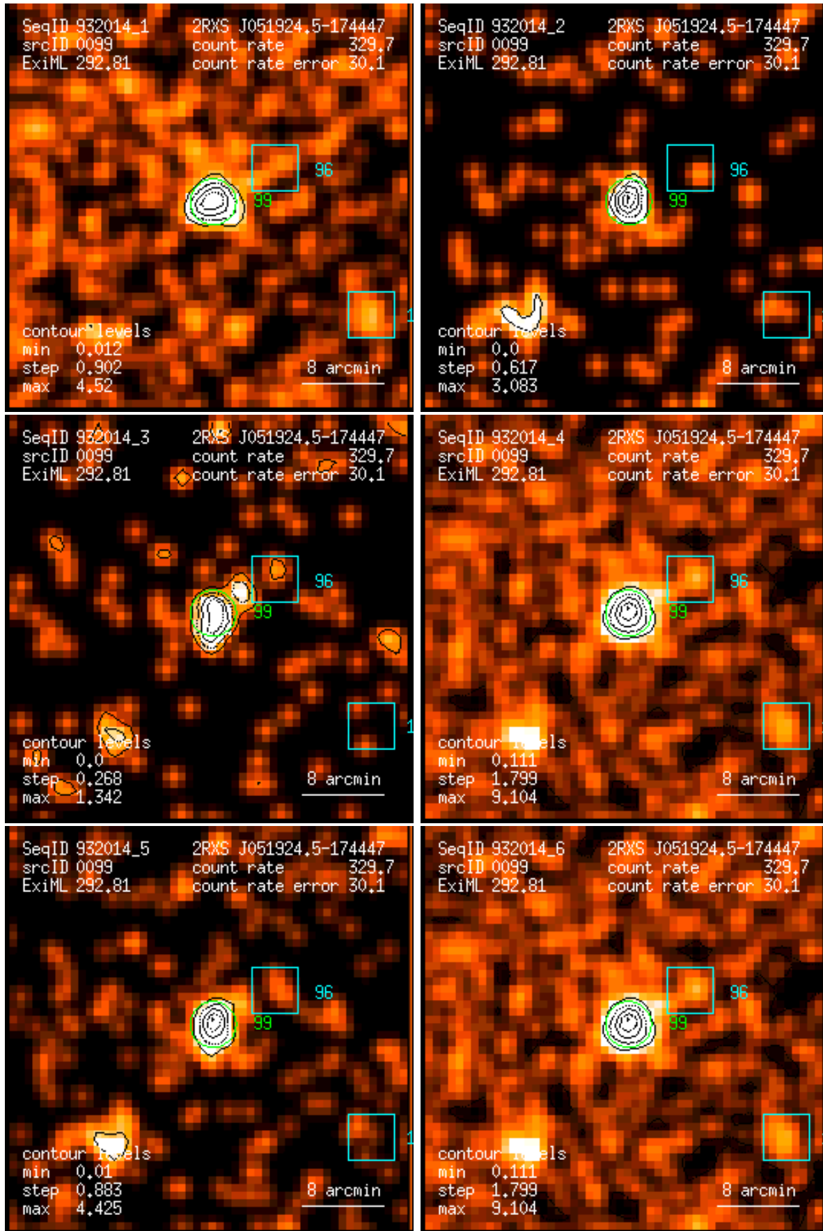
Figure 99: RASS 932014: detection 0099: band rate images, Gaussian filter: (1) PSPC channels 11 – 41, (2) 52 – 90, (3) 91 – 201, (4) 11 – 235, (5) 52 – 201, (6) 11 – 201. Broad band rates in counts/ks. Band rate contour levels in counts/ks/arcmin 2 .
