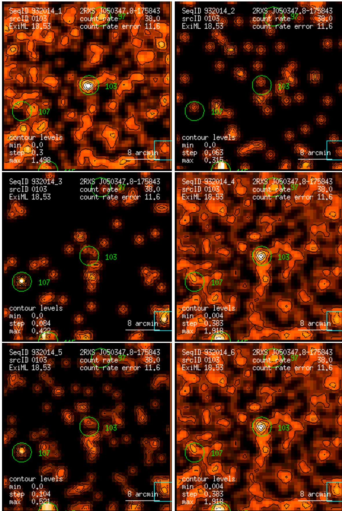
Figure 103: RASS 932014: detection 0103: band rate images, Gaussian filter: (1) PSPC channels 11 – 41, (2) 52 – 90, (3) 91 – 201, (4) 11 – 235, (5) 52 – 201, (6) 11 – 201. Broad band rates in counts/ks. Band rate contour levels in counts/ks/arcmin 2 .
