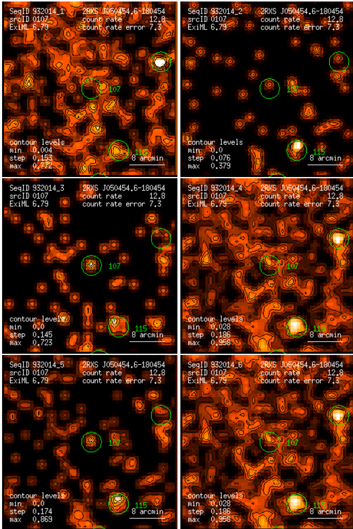
Figure 107: RASS 932014: detection 0107: band rate images, Gaussian filter: (1) PSPC channels 11 – 41, (2) 52 – 90, (3) 91 – 201, (4) 11 – 235, (5) 52 – 201, (6) 11 – 201. Broad band rates in counts/ks. Band rate contour levels in counts/ks/arcmin 2 .
