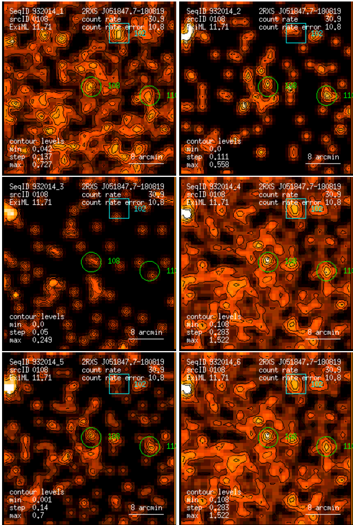
Figure 108: RASS 932014: detection 0108: band rate images, Gaussian filter: (1) PSPC channels 11 – 41, (2) 52 – 90, (3) 91 – 201, (4) 11 – 235, (5) 52 – 201, (6) 11 – 201. Broad band rates in counts/ks. Band rate contour levels in counts/ks/arcmin 2 .
