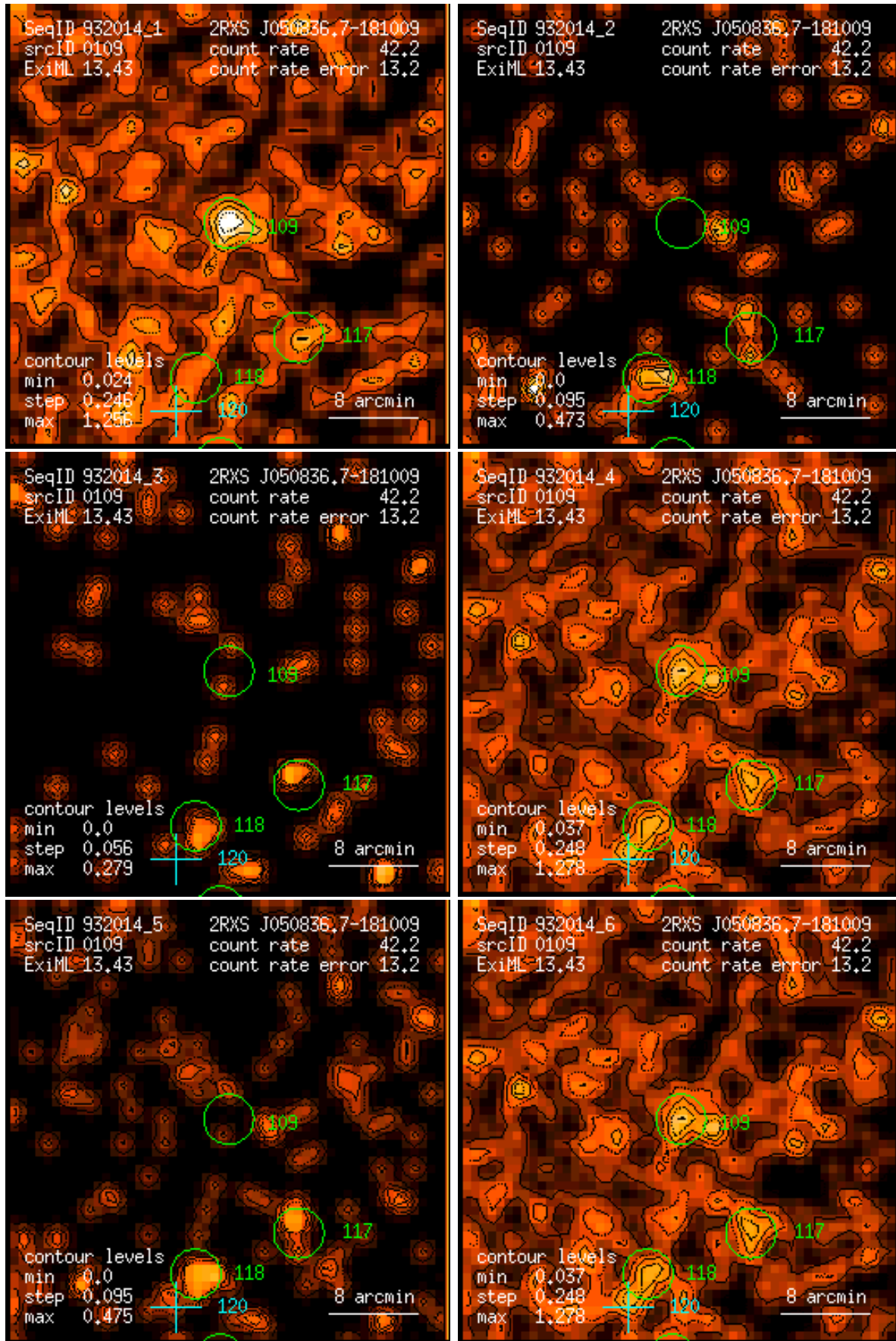
Figure 109: RASS 932014: detection 0109: band rate images, Gaussian filter: (1) PSPC channels 11 – 41, (2) 52 – 90, (3) 91 – 201, (4) 11 – 235, (5) 52 – 201, (6) 11 – 201. Broad band rates in counts/ks. Band rate contour levels in counts/ks/arcmin 2 .
