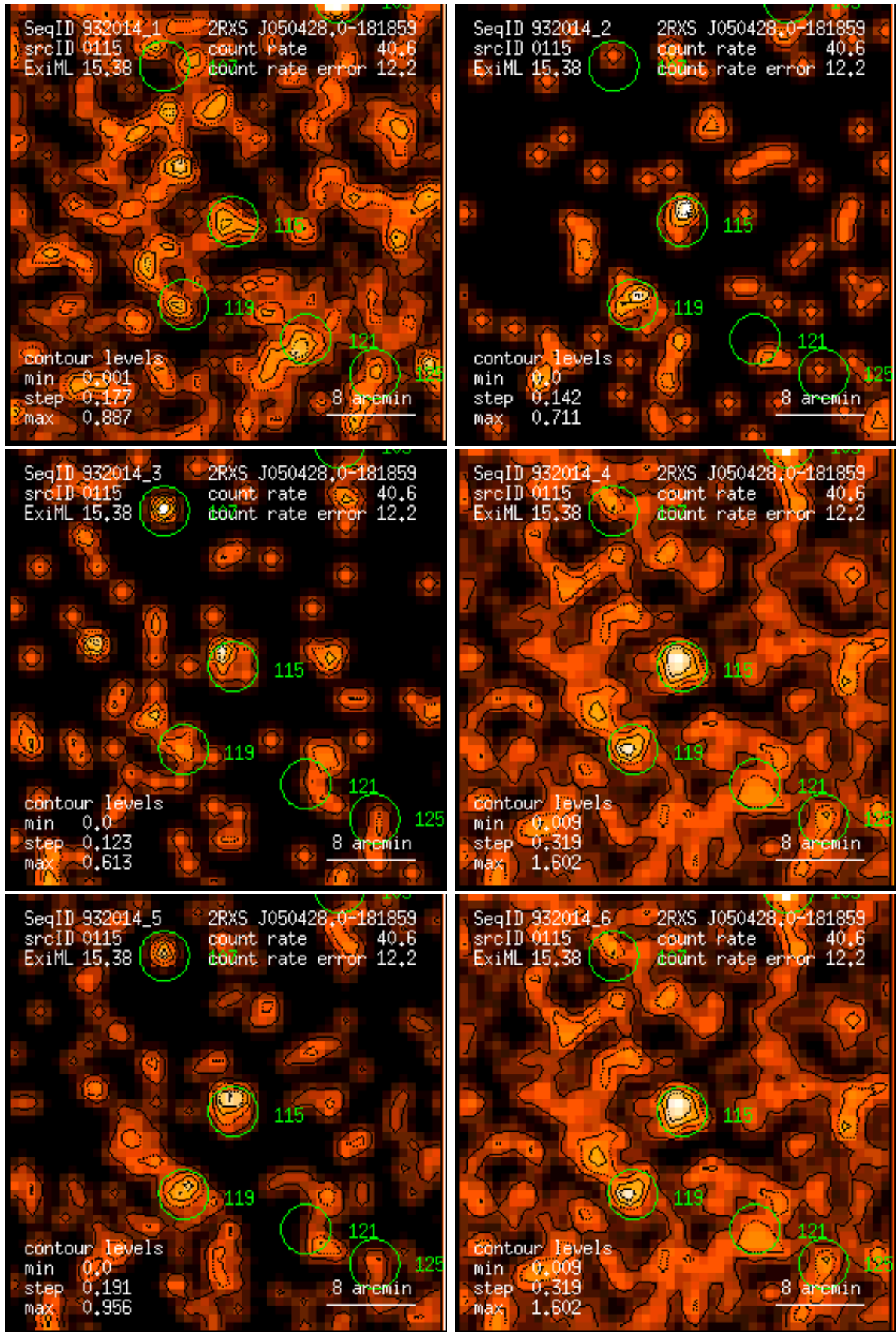
Figure 115: RASS 932014: detection 0115: band rate images, Gaussian filter: (1) PSPC channels 11 – 41, (2) 52 – 90, (3) 91 – 201, (4) 11 – 235, (5) 52 – 201, (6) 11 – 201. Broad band rates in counts/ks. Band rate contour levels in counts/ks/arcmin 2 .
