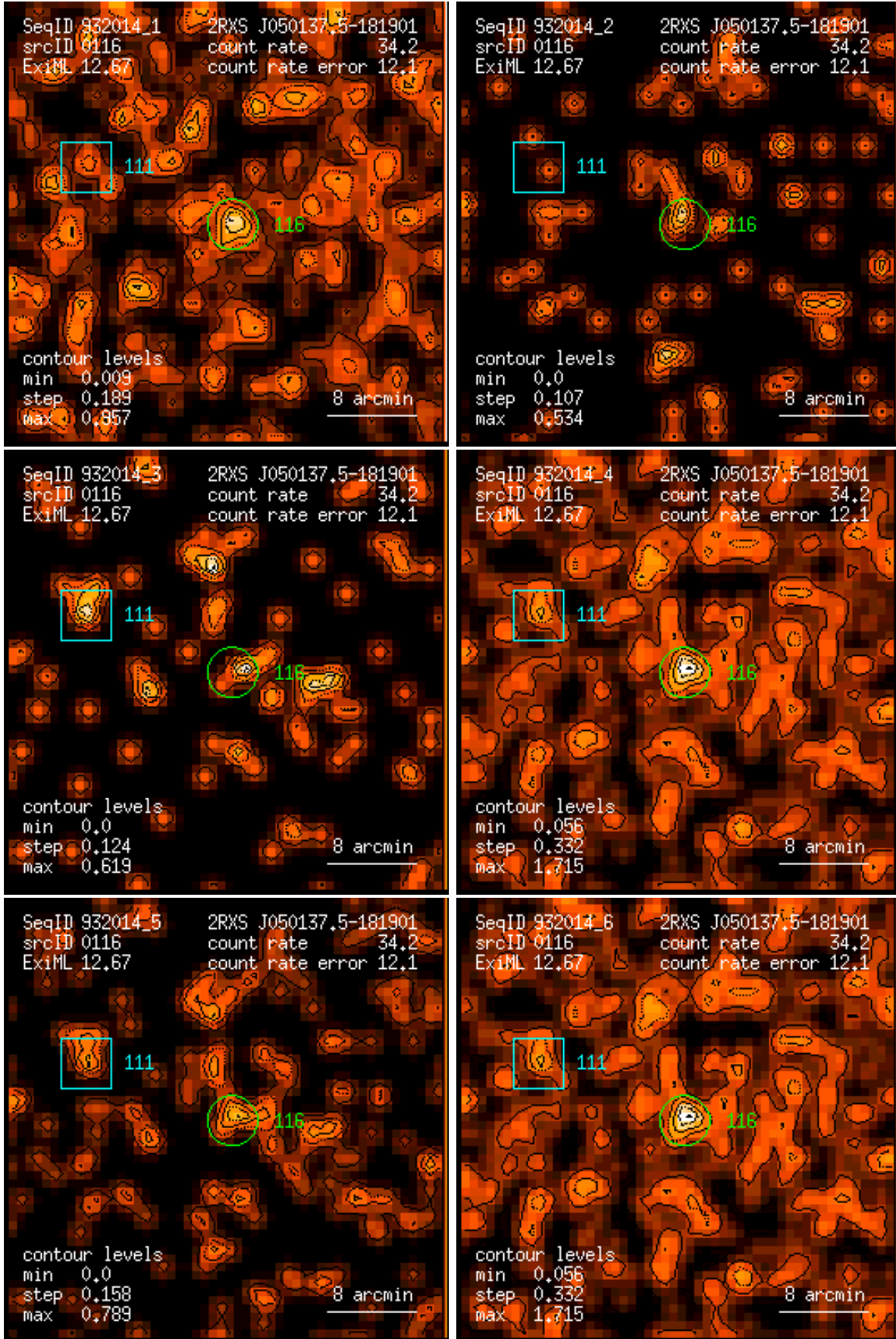
Figure 116: RASS 932014: detection 0116: band rate images, Gaussian filter: (1) PSPC channels 11 – 41, (2) 52 – 90, (3) 91 – 201, (4) 11 – 235, (5) 52 – 201, (6) 11 – 201. Broad band rates in counts/ks. Band rate contour levels in counts/ks/arcmin 2 .
