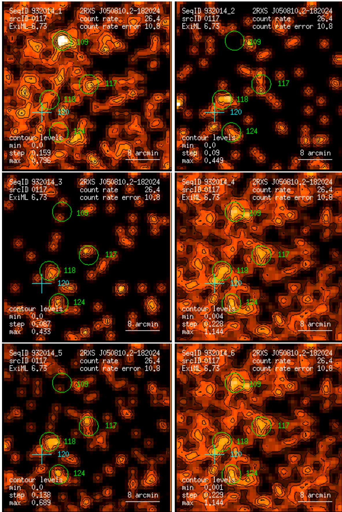
Figure 117: RASS 932014: detection 0117: band rate images, Gaussian filter: (1) PSPC channels 11 – 41, (2) 52 – 90, (3) 91 – 201, (4) 11 – 235, (5) 52 – 201, (6) 11 – 201. Broad band rates in counts/ks. Band rate contour levels in counts/ks/arcmin 2 .
