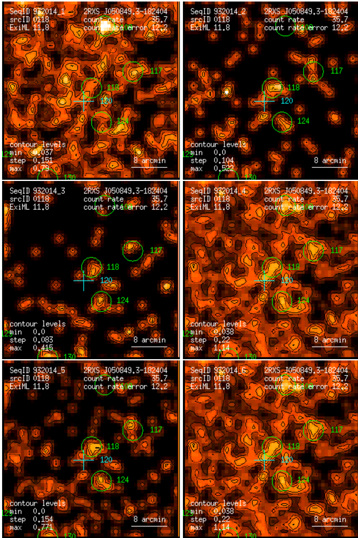
Figure 118: RASS 932014: detection 0118: band rate images, Gaussian filter: (1) PSPC channels 11 – 41, (2) 52 – 90, (3) 91 – 201, (4) 11 – 235, (5) 52 – 201, (6) 11 – 201. Broad band rates in counts/ks. Band rate contour levels in counts/ks/arcmin 2 .
