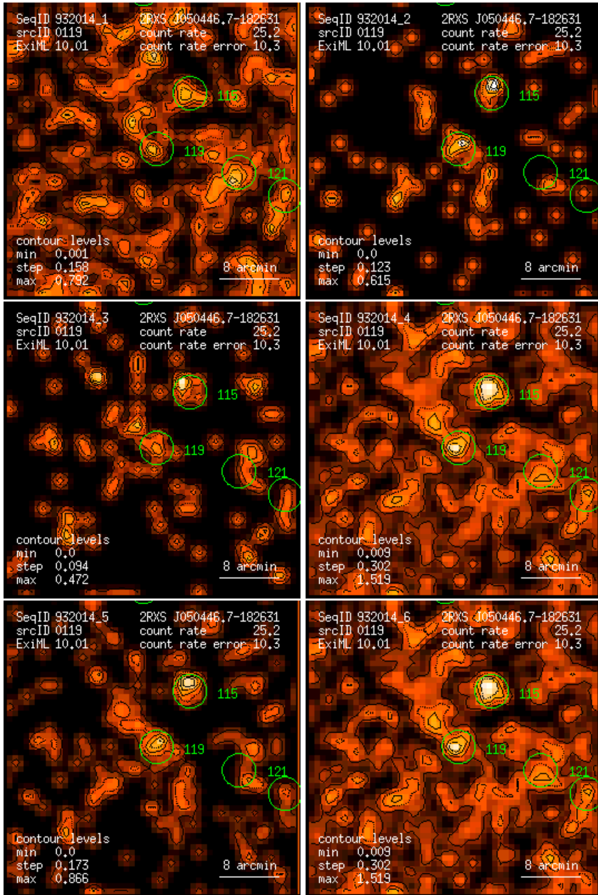
Figure 119: RASS 932014: detection 0119: band rate images, Gaussian filter: (1) PSPC channels 11 – 41, (2) 52 – 90, (3) 91 – 201, (4) 11 – 235, (5) 52 – 201, (6) 11 – 201. Broad band rates in counts/ks. Band rate contour levels in counts/ks/arcmin 2 .
