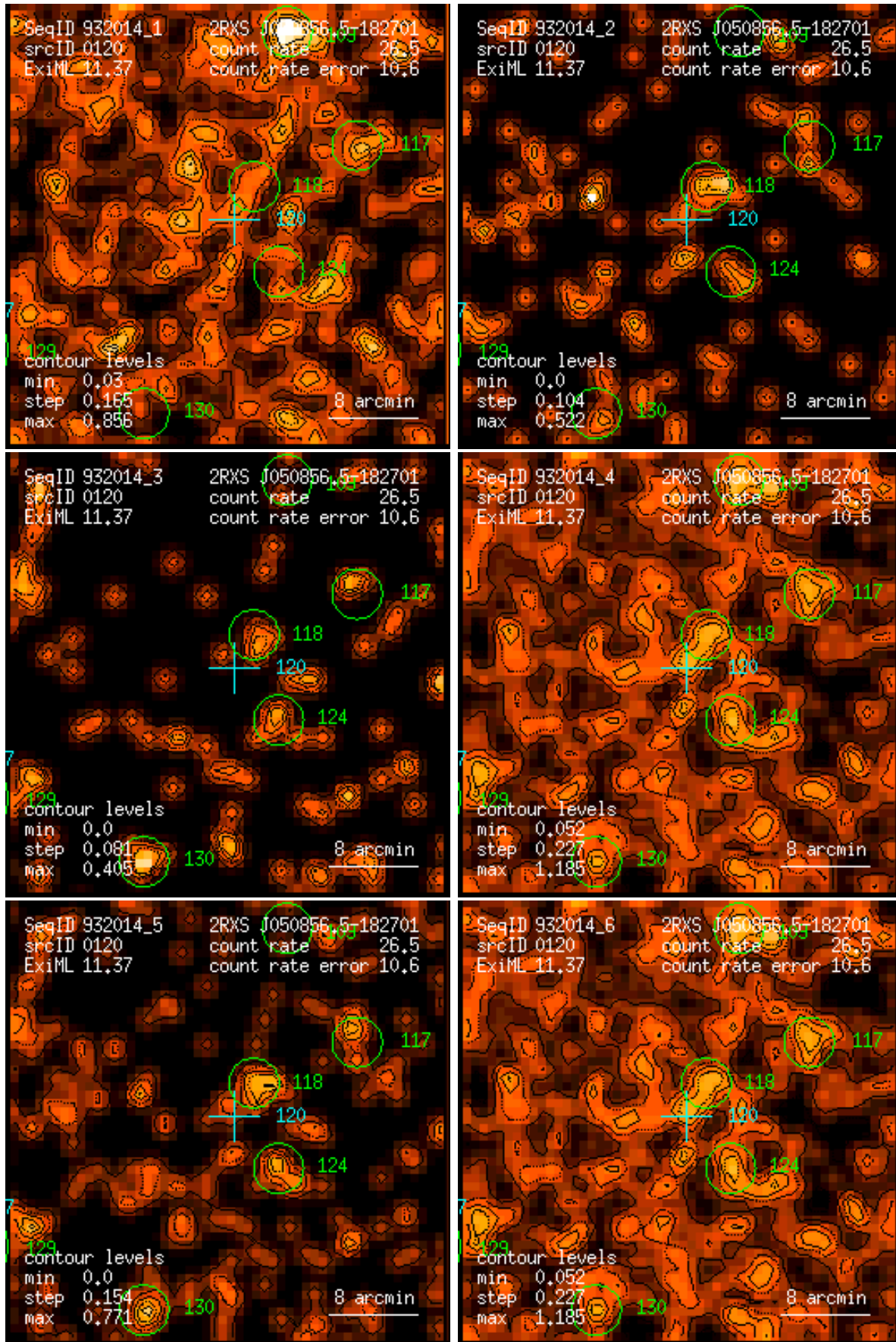
Figure 120: RASS 932014: detection 0120: band rate images, Gaussian filter: (1) PSPC channels 11 – 41, (2) 52 – 90, (3) 91 – 201, (4) 11 – 235, (5) 52 – 201, (6) 11 – 201. Broad band rates in counts/ks. Band rate contour levels in counts/ks/arcmin 2 .
