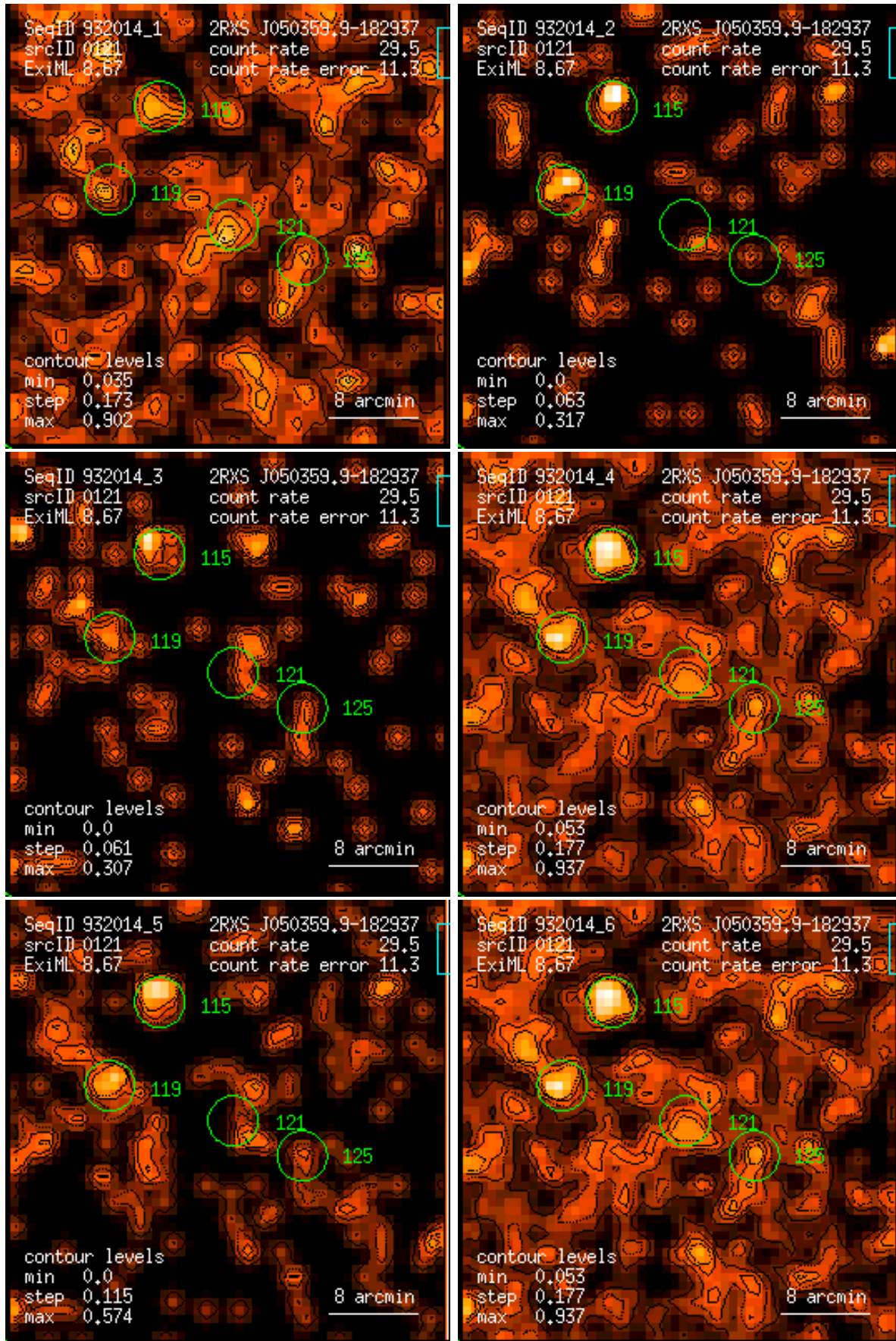
Figure 121: RASS 932014: detection 0121: band rate images, Gaussian filter: (1) PSPC channels 11 – 41, (2) 52 – 90, (3) 91 – 201, (4) 11 – 235, (5) 52 – 201, (6) 11 – 201. Broad band rates in counts/ks. Band rate contour levels in counts/ks/arcmin 2 .
