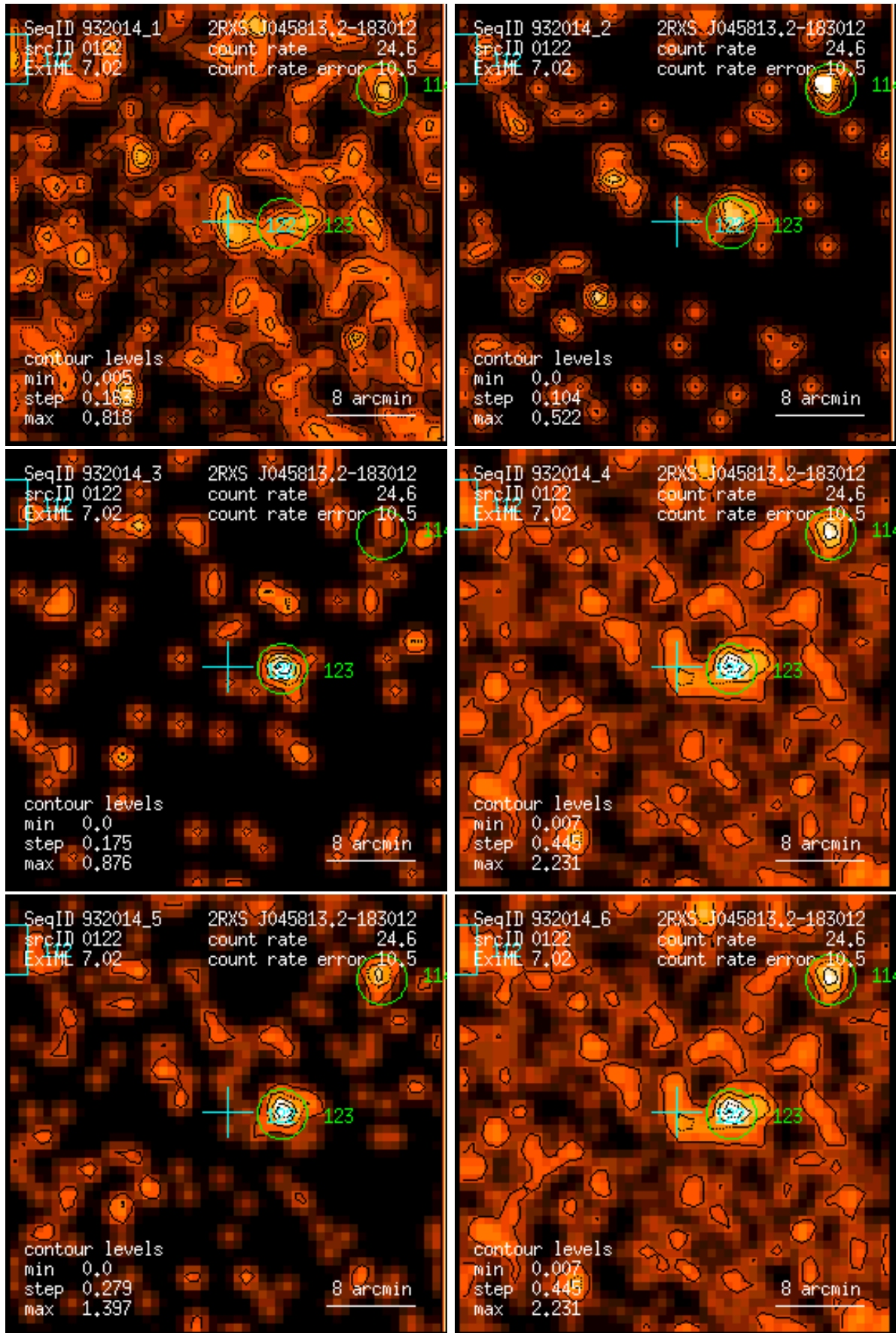
Figure 122: RASS 932014: detection 0122: band rate images, Gaussian filter: (1) PSPC channels 11 – 41, (2) 52 – 90, (3) 91 – 201, (4) 11 – 235, (5) 52 – 201, (6) 11 – 201. Broad band rates in counts/ks. Band rate contour levels in counts/ks/arcmin 2 .
