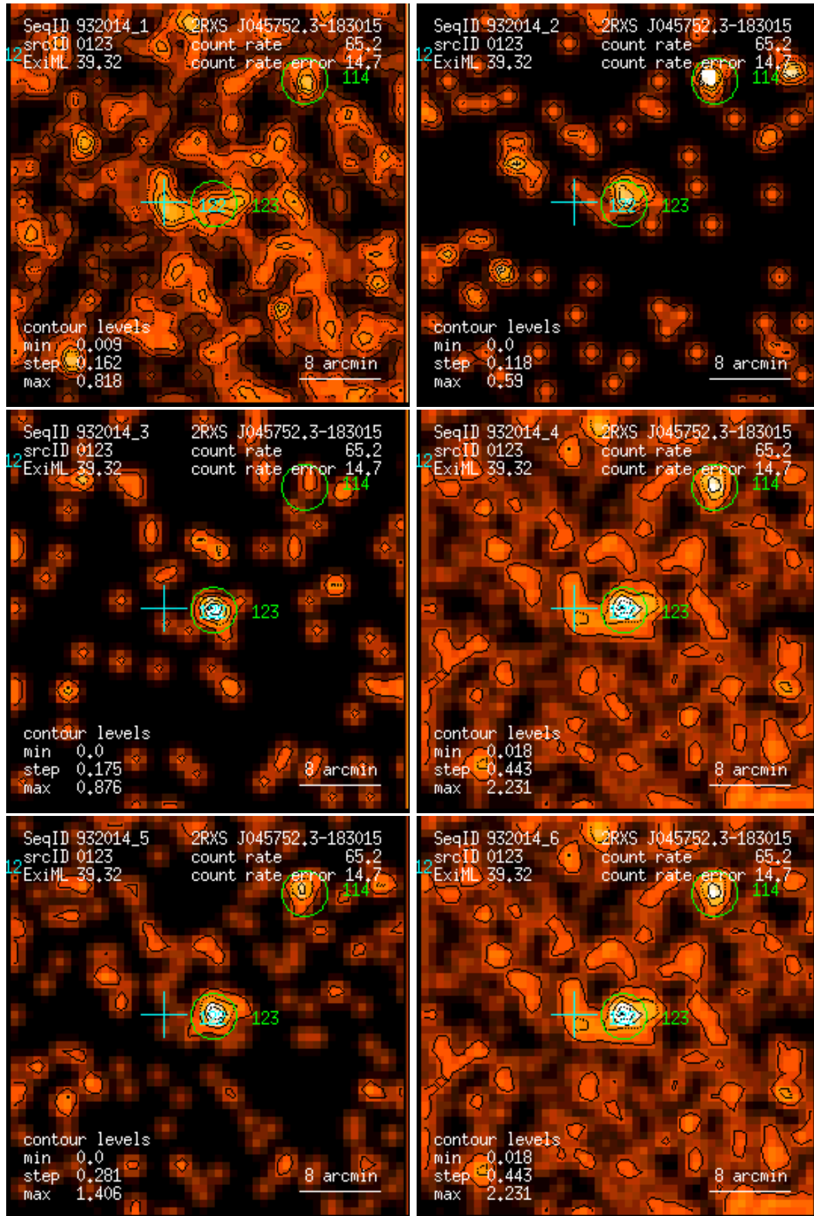
Figure 123: RASS 932014: detection 0123: band rate images, Gaussian filter: (1) PSPC channels 11 – 41, (2) 52 – 90, (3) 91 – 201, (4) 11 – 235, (5) 52 – 201, (6) 11 – 201. Broad band rates in counts/ks. Band rate contour levels in counts/ks/arcmin 2 .
